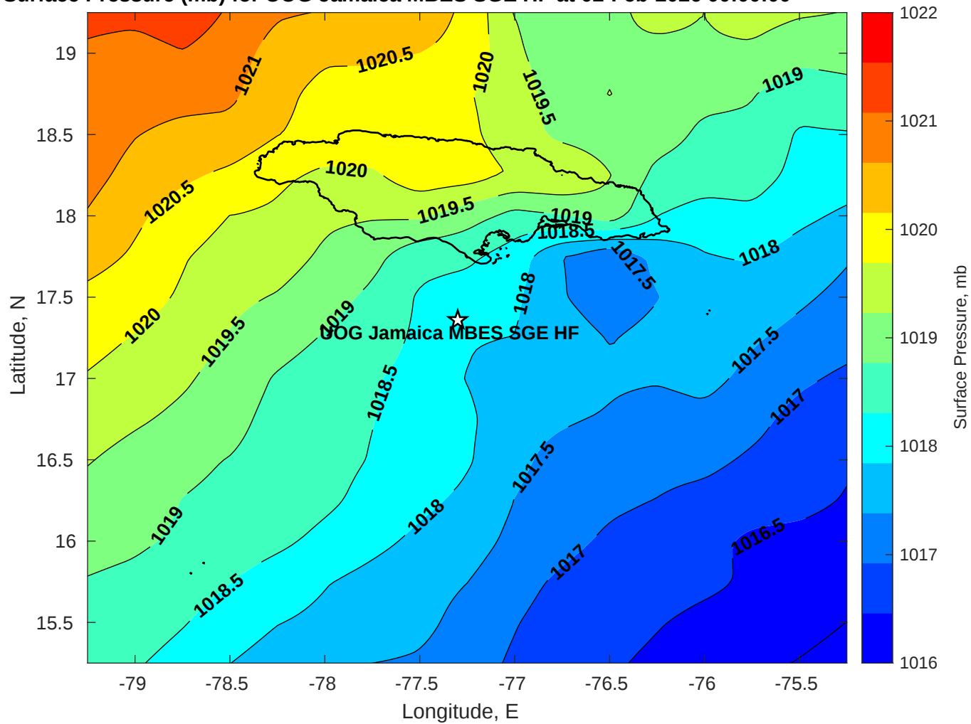
Surface Pressure (mb) for UOG Jamaica MBES SGE HF at 02-Feb-2026 00:00:00
