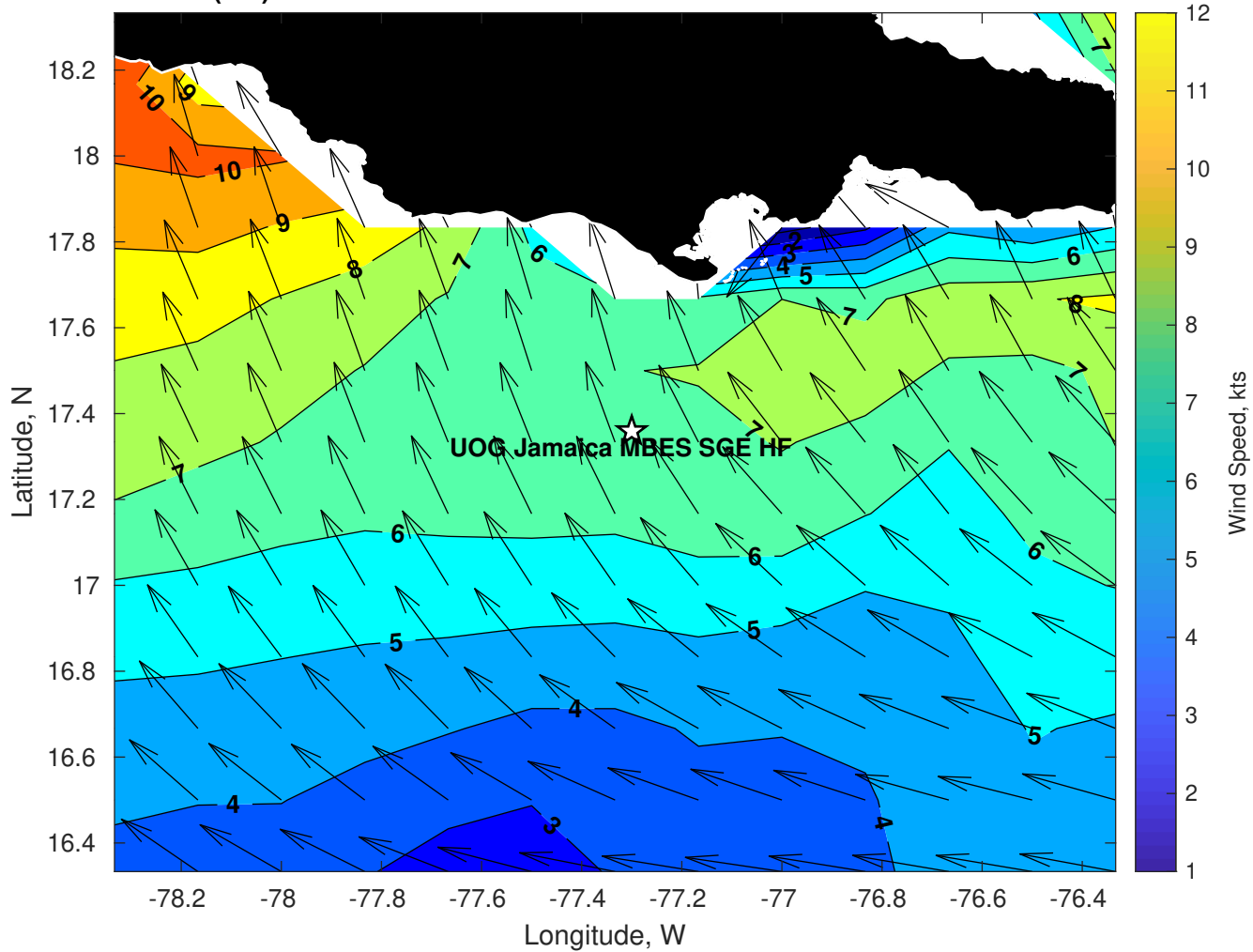
GFS Winds (kts) for UOG Jamaica MBES SGE HF at 31-Jan-2026 09:00:00
