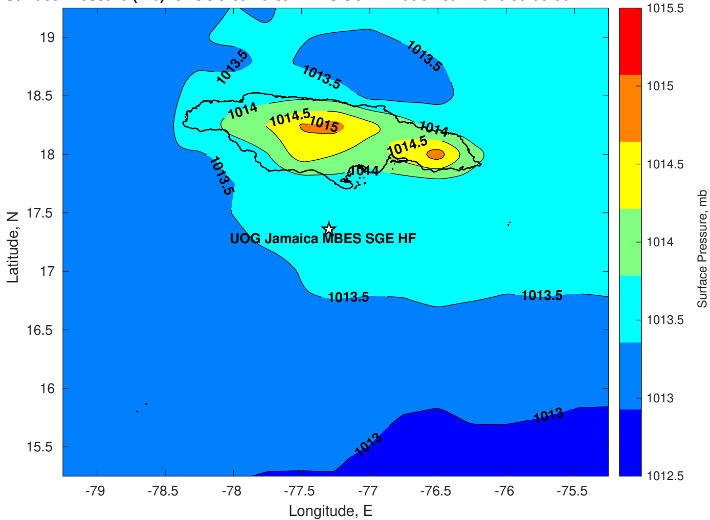
Surface Pressure (mb) for UOG Jamaica MBES SGE HF at 31-Jan-2026 00:00:00
