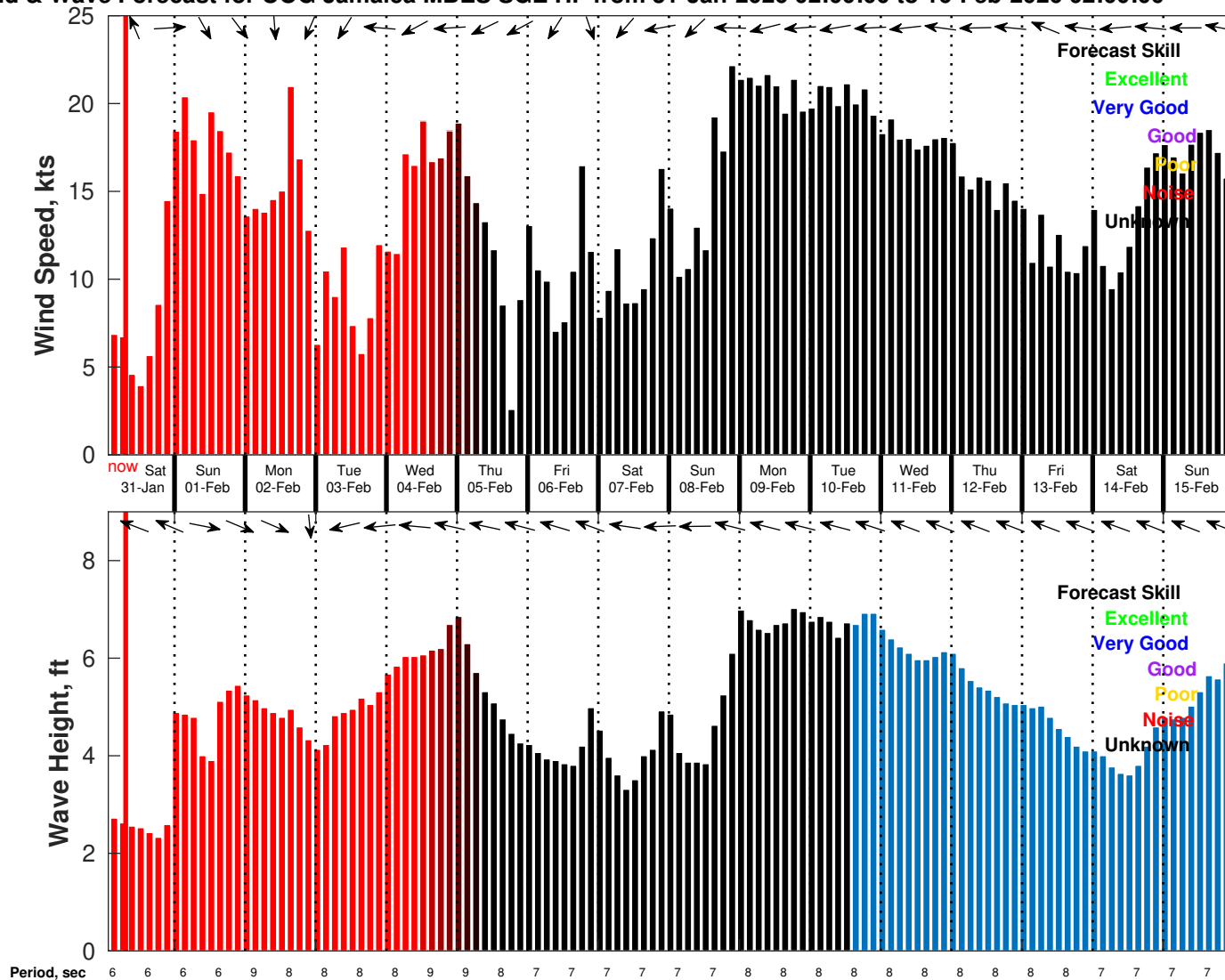
Wind & Wave Forecast for UOG Jamaica MBES SGE HF from 31-Jan-2026 02:00:00 to 16-Feb-2026 02:00:00
