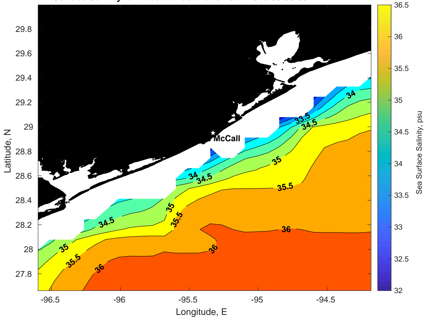
Surface Salinity for Brooks McCall at 31-Jan-2026 00:00:00
