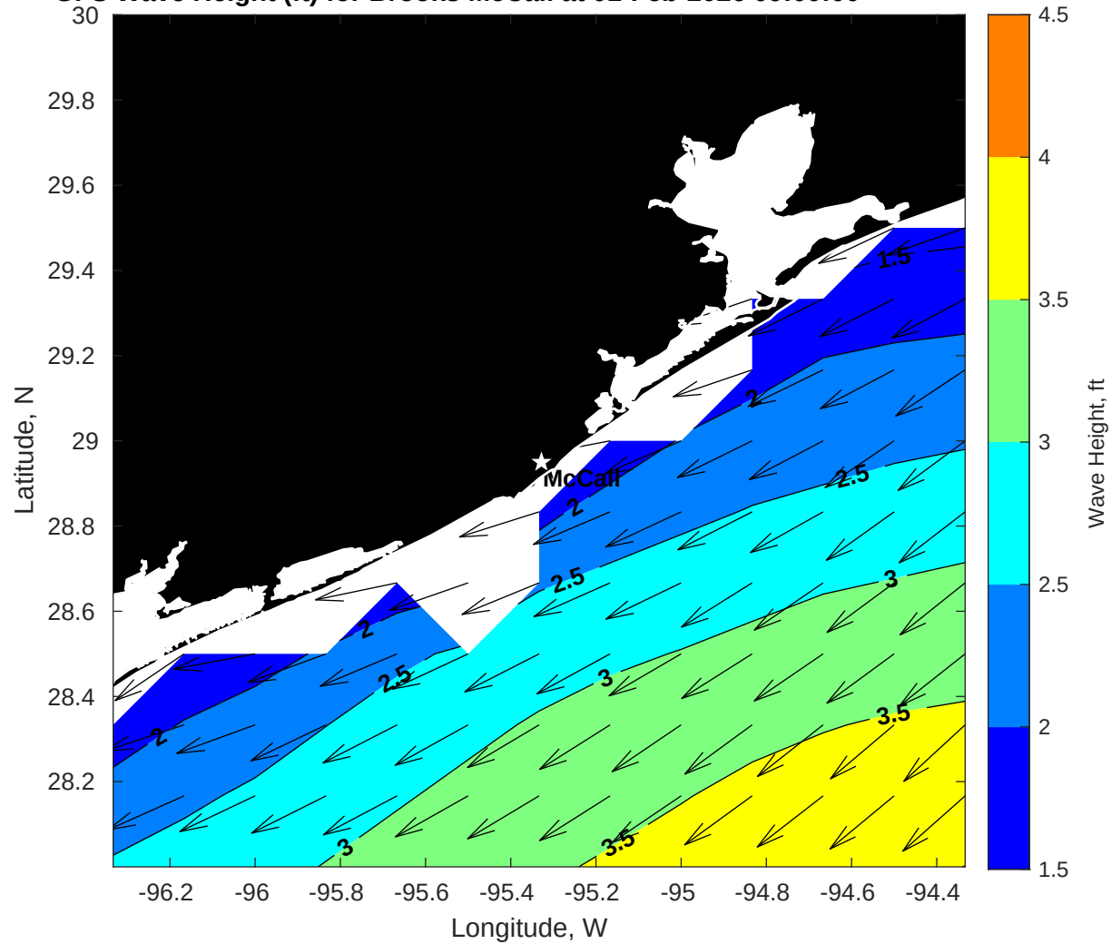
GFS Wave Height (ft) for Brooks McCall at 01-Feb-2026 09:00:00
