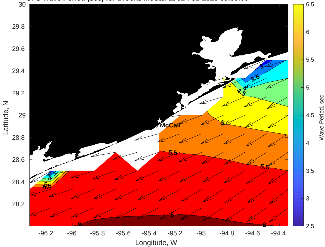
GFS Wave Period (sec) for Brooks McCall at 01-Feb-2026 09:00:00
