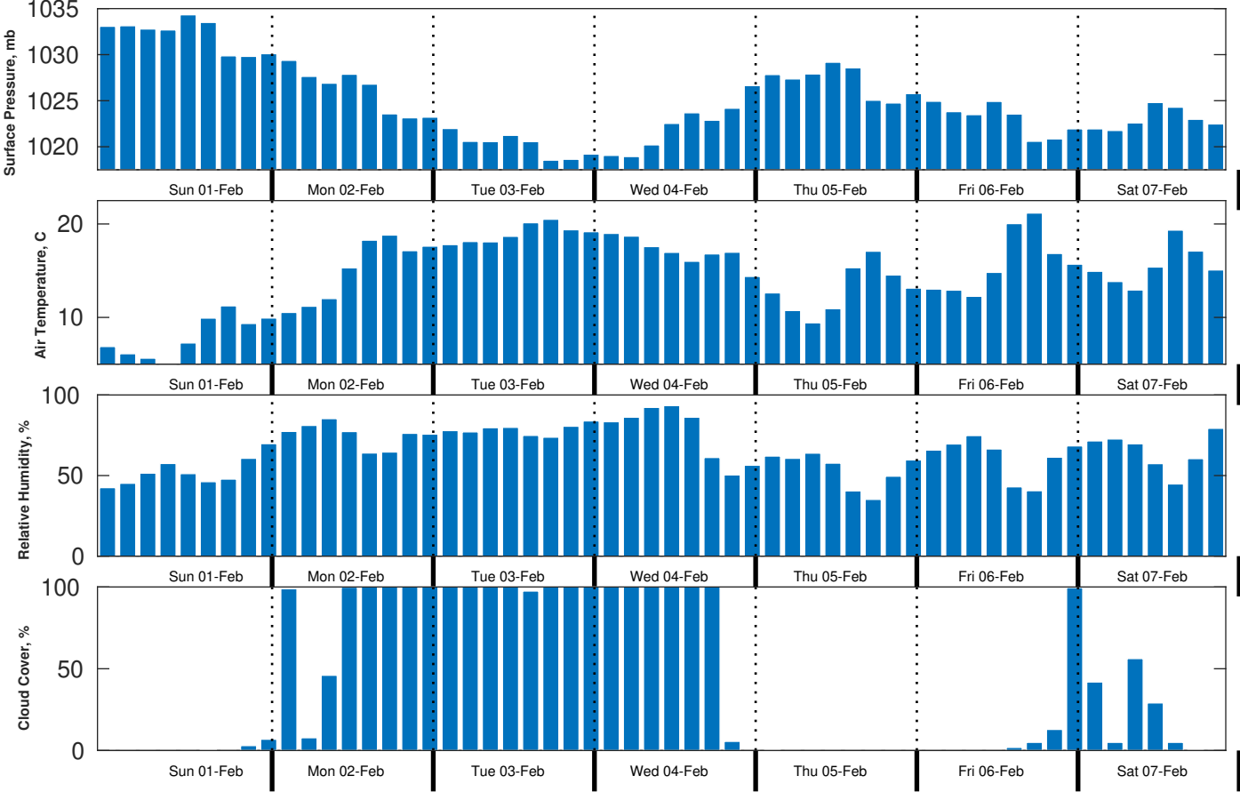
Met Forecast for Brooks McCall from 01-Feb-2026 00:00:00 to 08-Feb-2026 00:00:00
