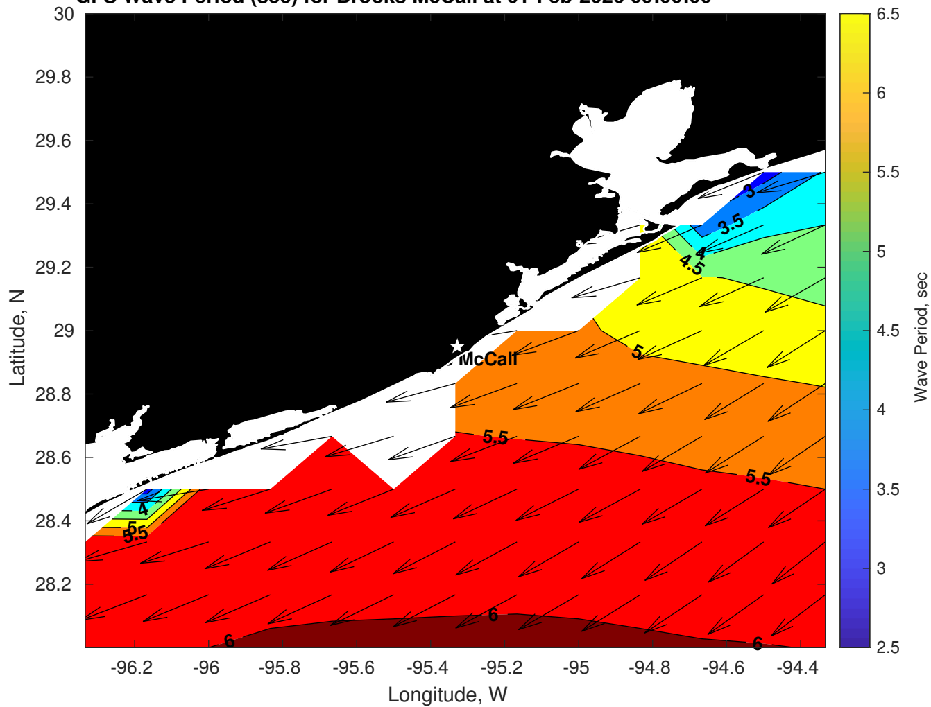
GFS Wave Period (sec) for Brooks McCall at 01-Feb-2026 09:00:00
