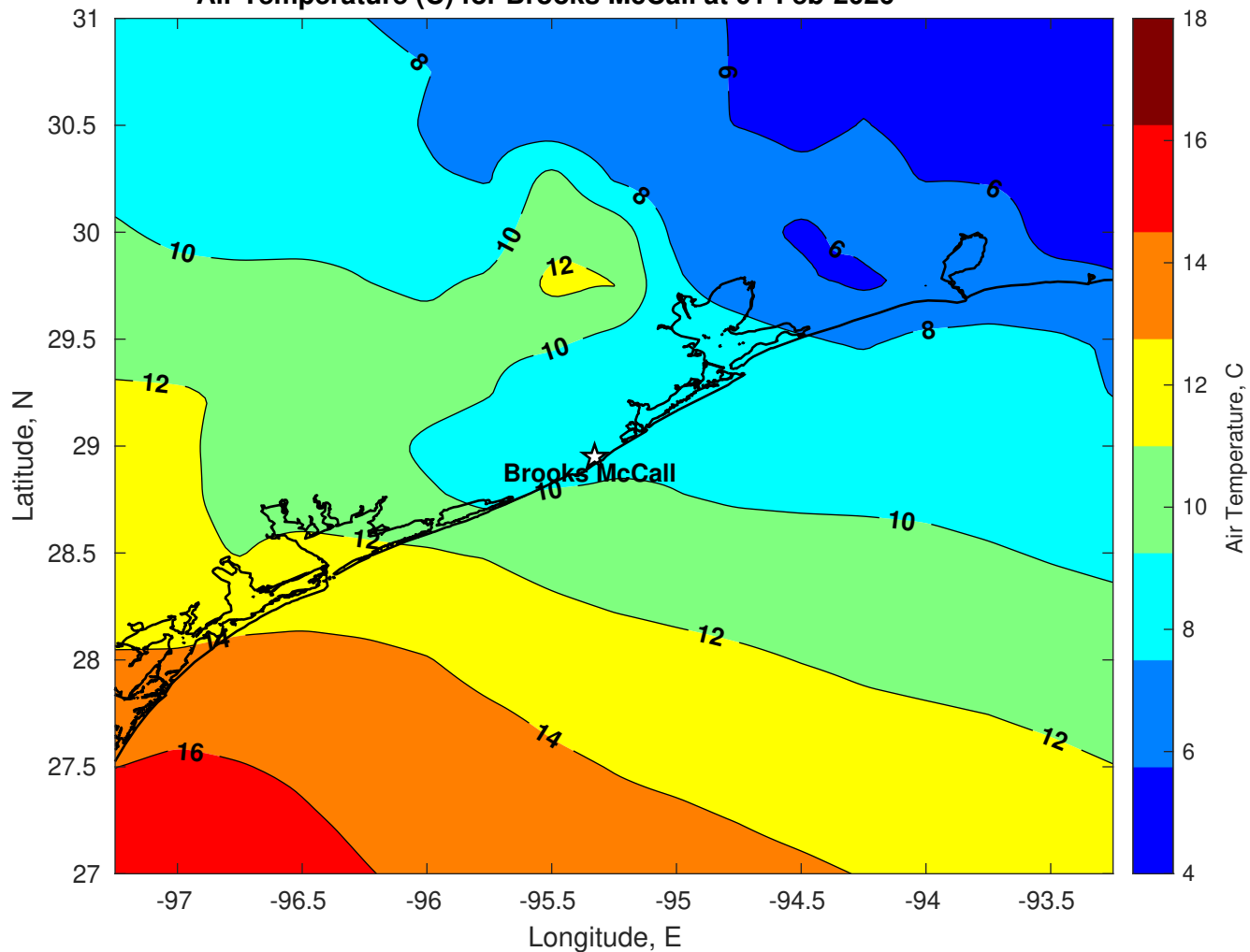
Air Temperature (C) for Brooks McCall at 01-Feb-2026
