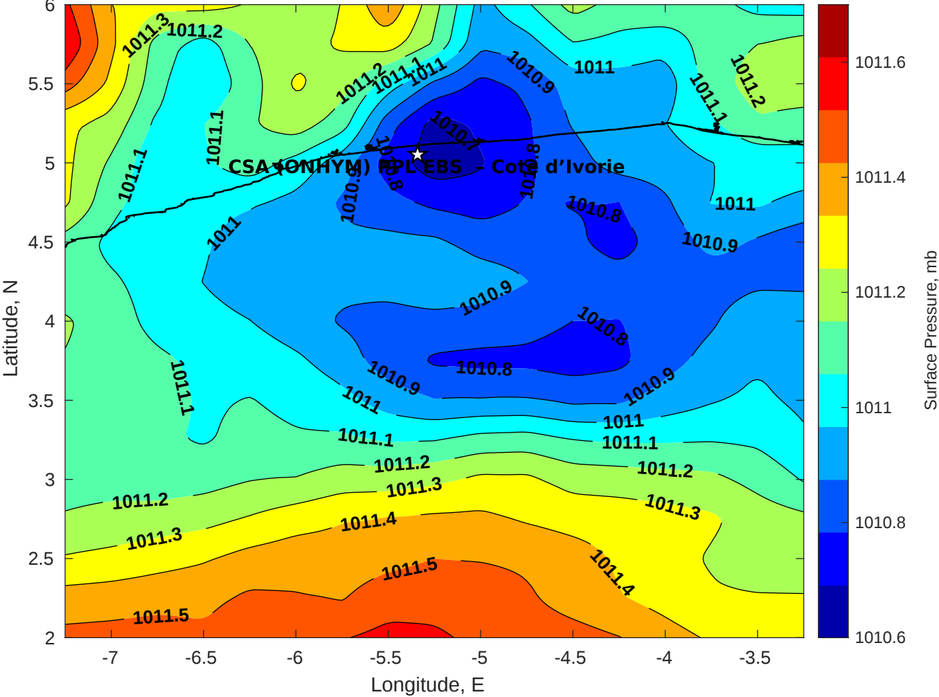
Surface Pressure (mb) for CSA (ONHYM) PPL EBS - Cote d'Ivoire at 02-Feb-2026 00:00:00
