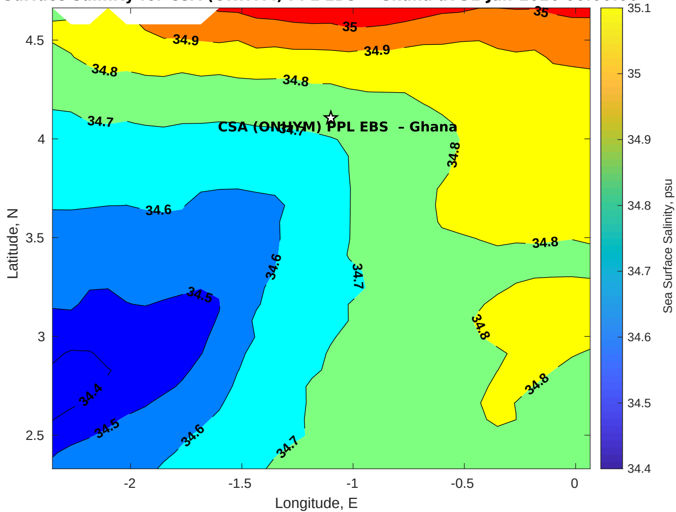
Surface Salinity for CSA (ONHYM) PPL EBS - Ghana at 31-Jan-2026 00:00:00
