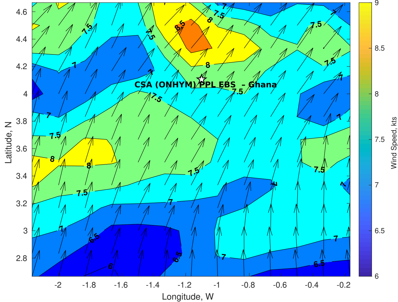
GFS Winds (kts) for CSA (ONHYM) PPL EBS - Ghana at 01-Feb-2026 09:00:00
