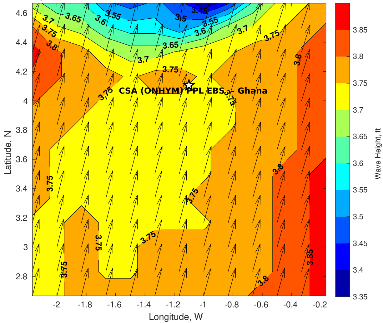
GFS Wave Height (ft) for CSA (ONHYM) PPL EBS - Ghana at 01-Feb-2026 09:00:00
