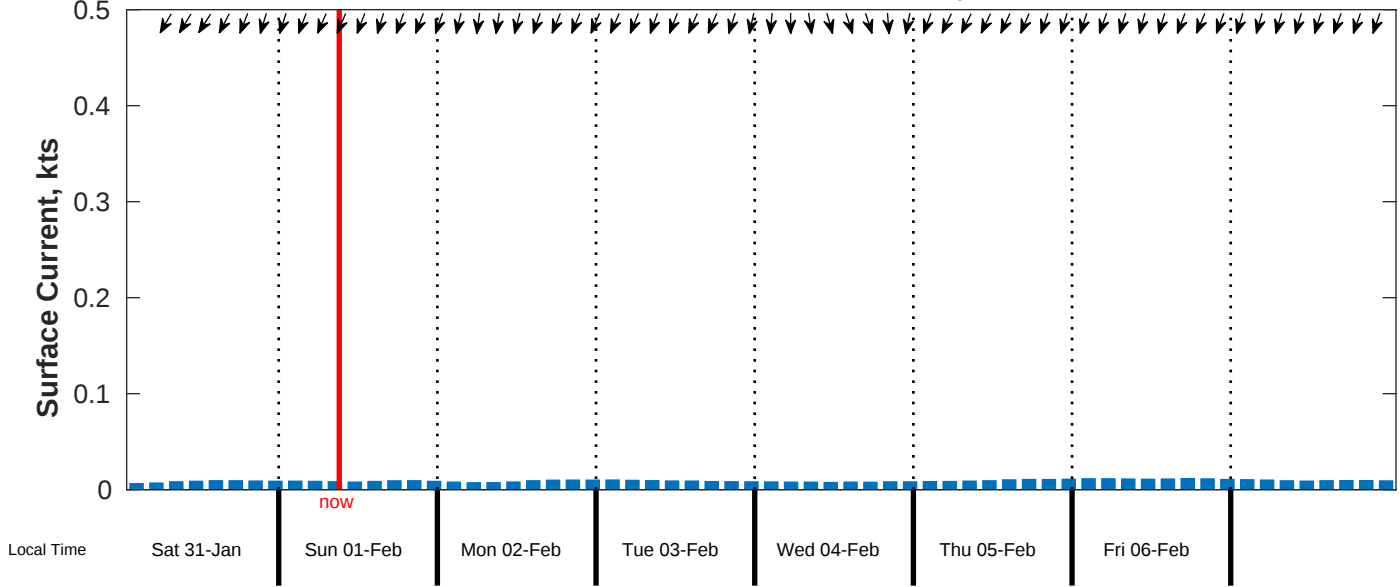
Surface Current Forecast for CSA (ONHYM) PPL EBS - Ghana from 31-Jan-2026 00:00:00 to 08-Feb-2026 00:00:00
