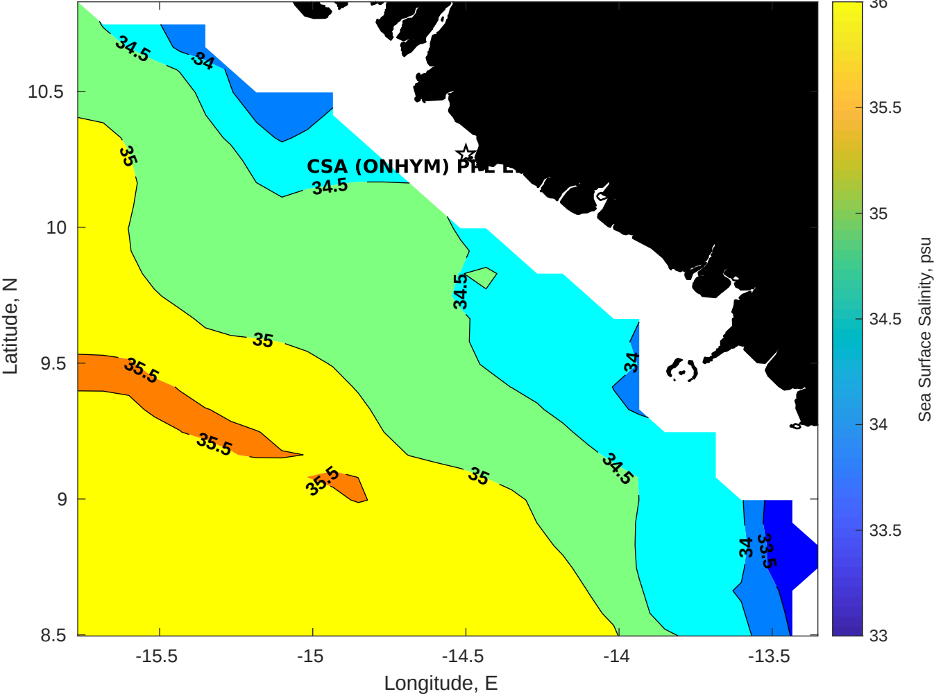
Surface Salinity for CSA (ONHYM) PPL EBS - Guinea at 31-Jan-2026 00:00:00
