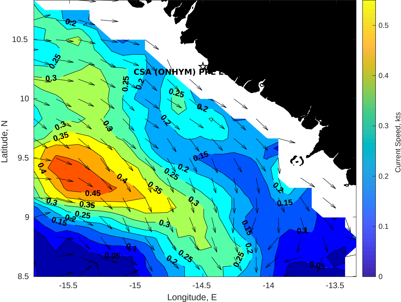
Surface Currents for CSA (ONHYM) PPL EBS - Guinea at 31-Jan-2026 00:00:00
