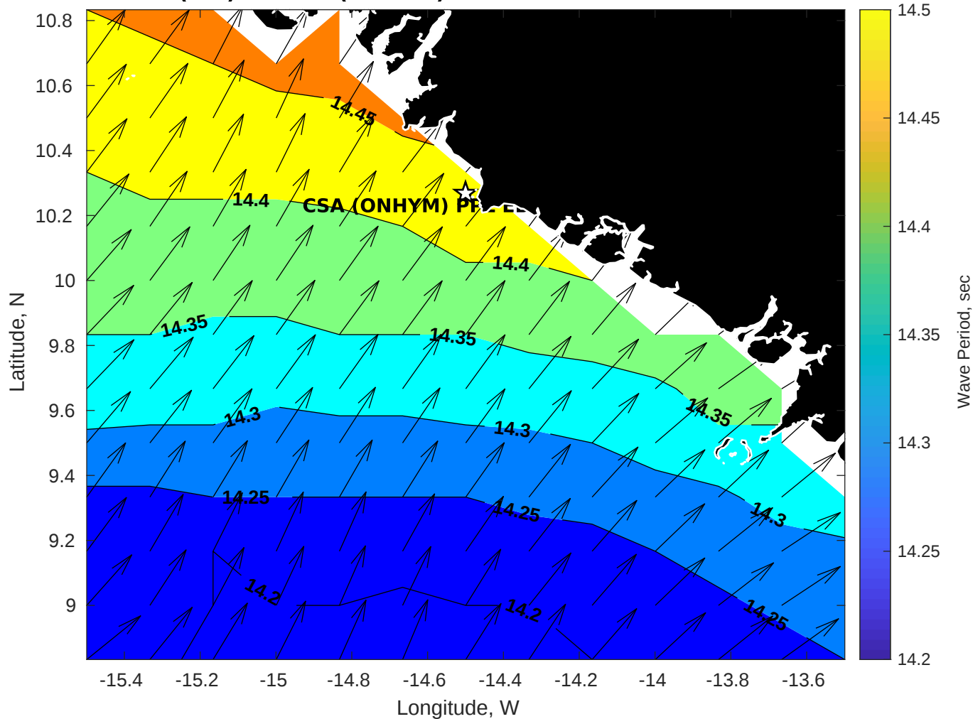
GFS Wave Period (sec) for CSA (ONHYM) PPL EBS - Guinea at 01-Feb-2026 09:00:00
