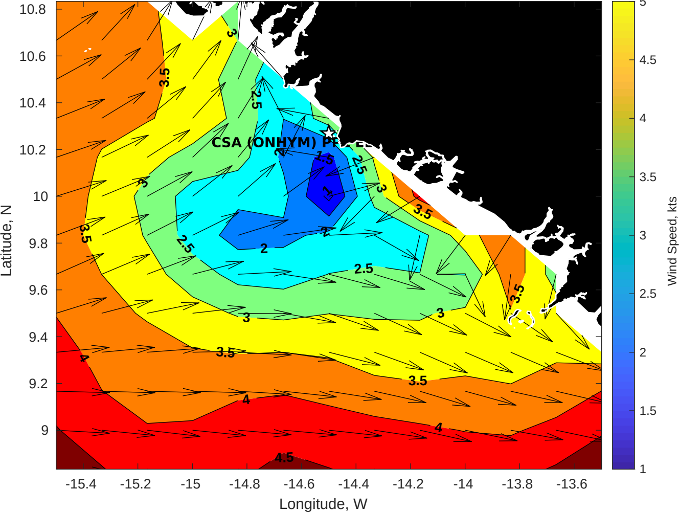
GFS Winds (kts) for CSA (ONHYM) PPL EBS - Guinea at 01-Feb-2026 09:00:00
