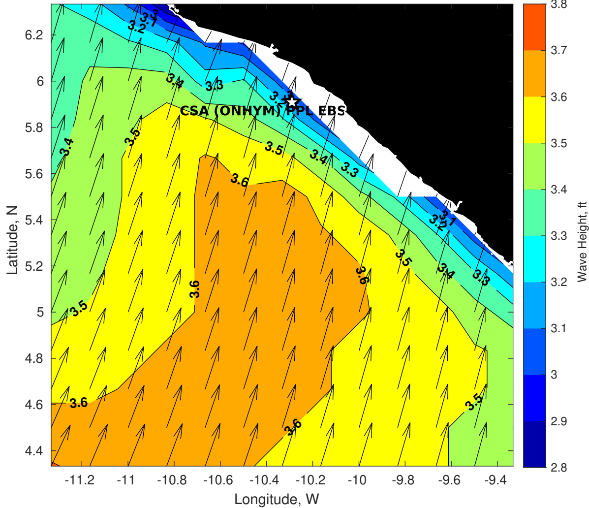
GFS Wave Height (ft) for CSA (ONHYM) PPL EBS - Liberia at 01-Feb-2026 09:00:00
