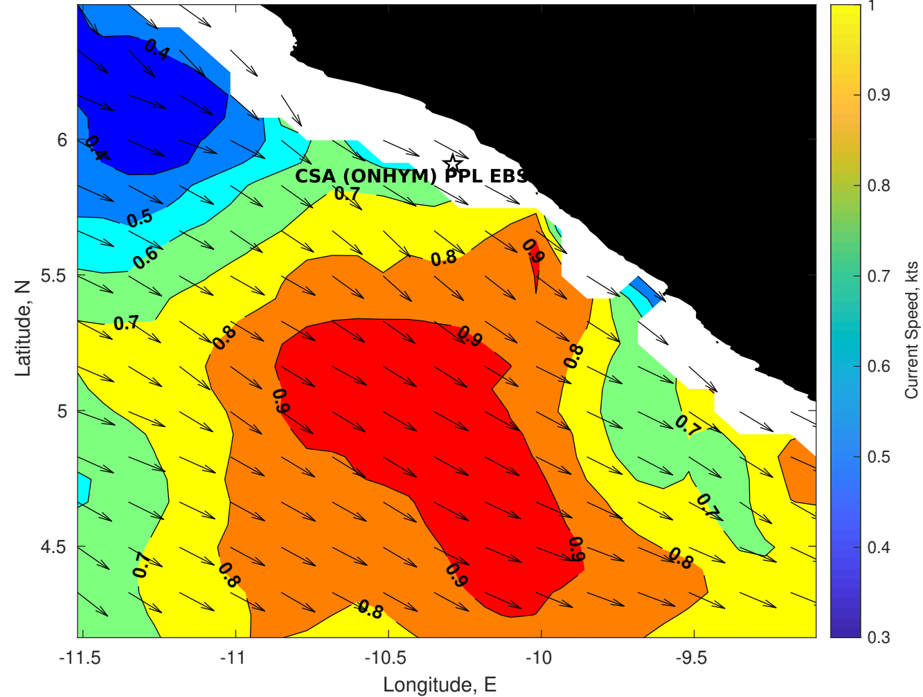
Surface Currents for CSA (ONHYM) PPL EBS - Liberia at 31-Jan-2026 00:00:00
