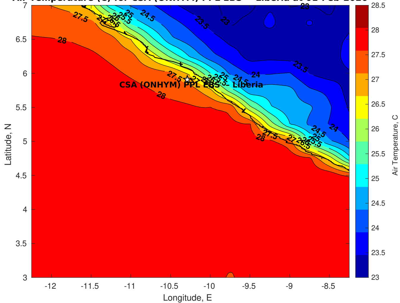
Air Temperature (C) for CSA (ONHYM) PPL EBS - Liberia at 01-Feb-2026
