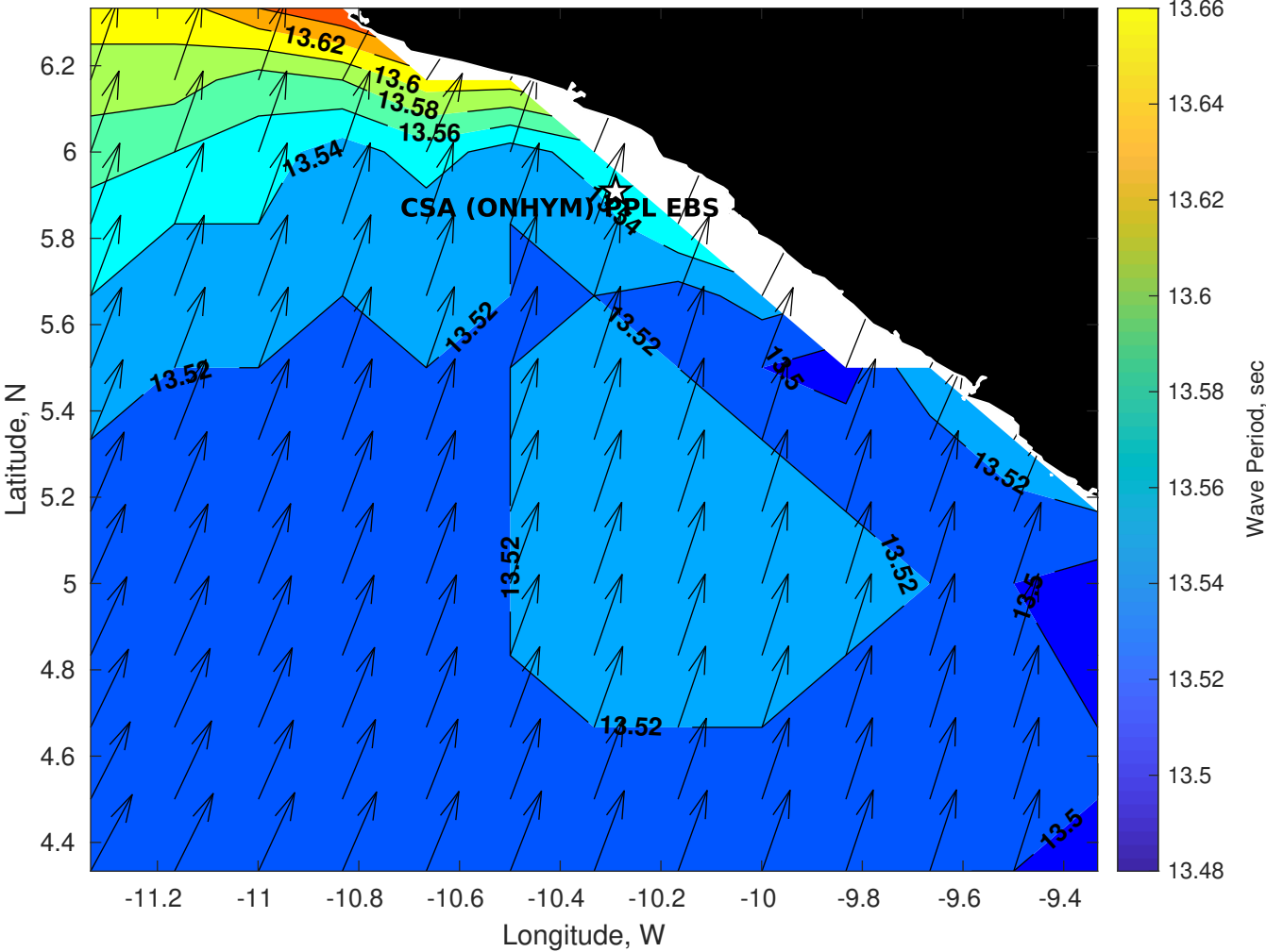
GFS Wave Period (sec) for CSA (ONHYM) PPL EBS - Liberia at 01-Feb-2026 09:00:00
