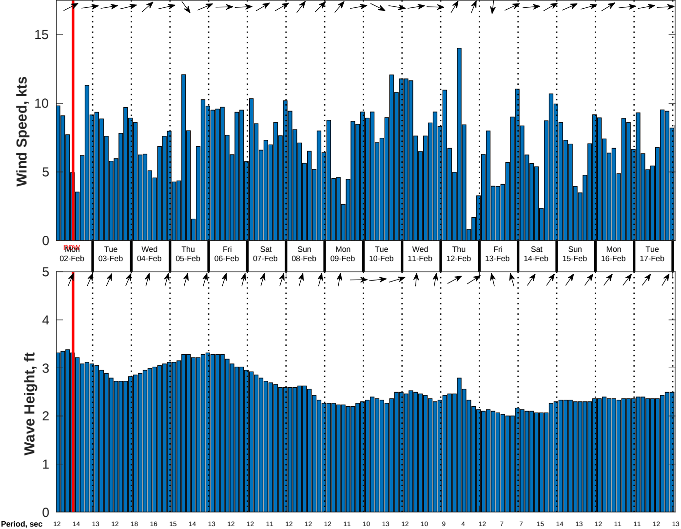
Wind & Wave Forecast for CSA (ONHYM) PPL EBS - Liberia from 01-Feb-2026 01:00:00 to 17-Feb-2026 01:00:00
