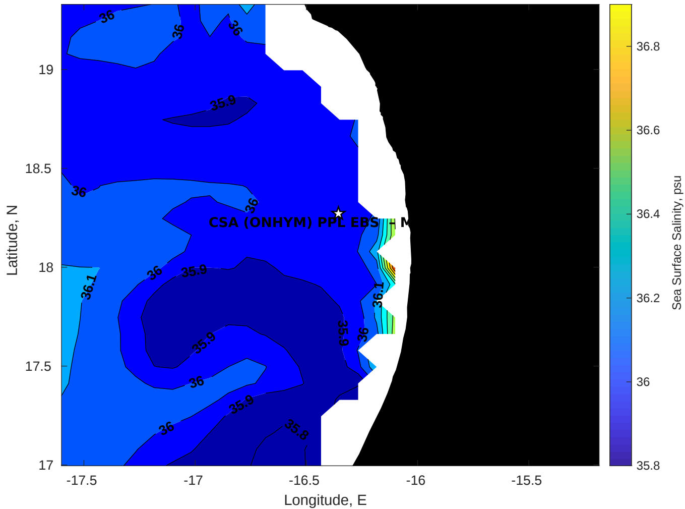
Surface Salinity for CSA (ONHYM) PPL EBS - Mauritania at 31-Jan-2026 00:00:00
