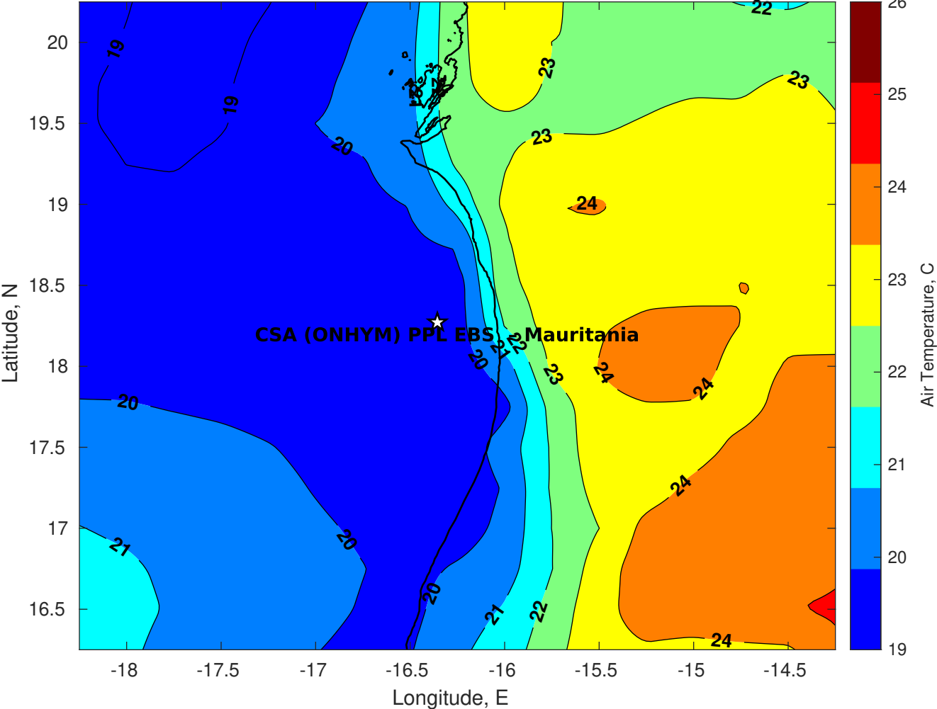
Air Temperature (C) for CSA (ONHYM) PPL EBS - Mauritania at 01-Feb-2026
