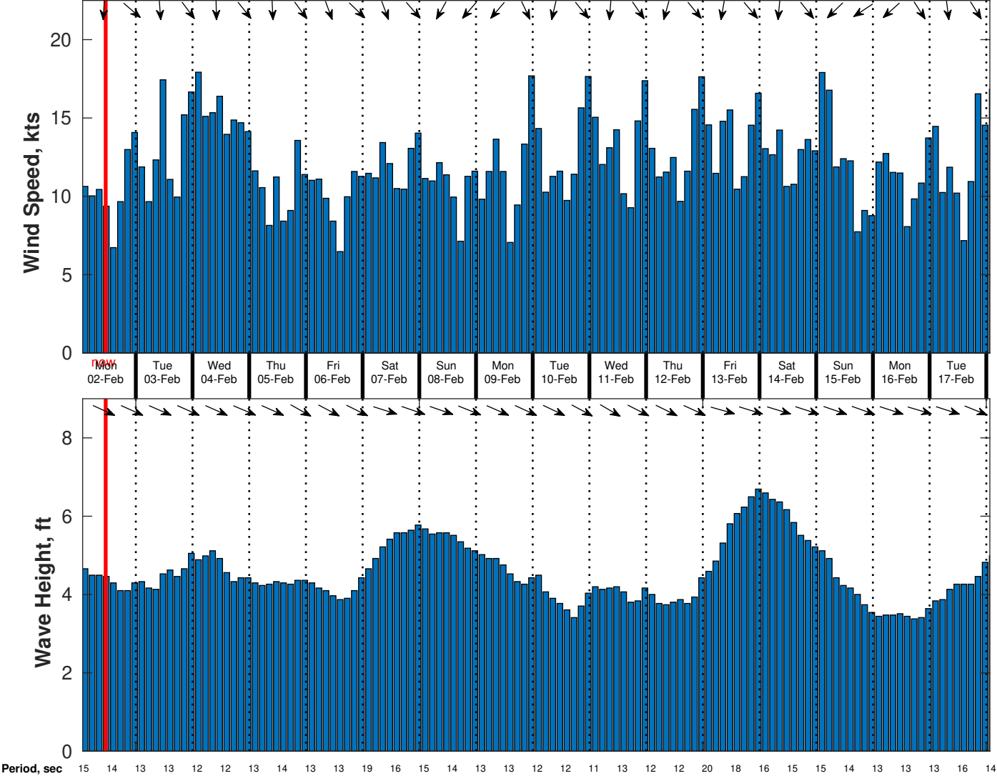
Wind & Wave Forecast for CSA (ONHYM) PPL EBS - Mauritania from 01-Feb-2026 01:00:00 to 17-Feb-2026 01:00:00
