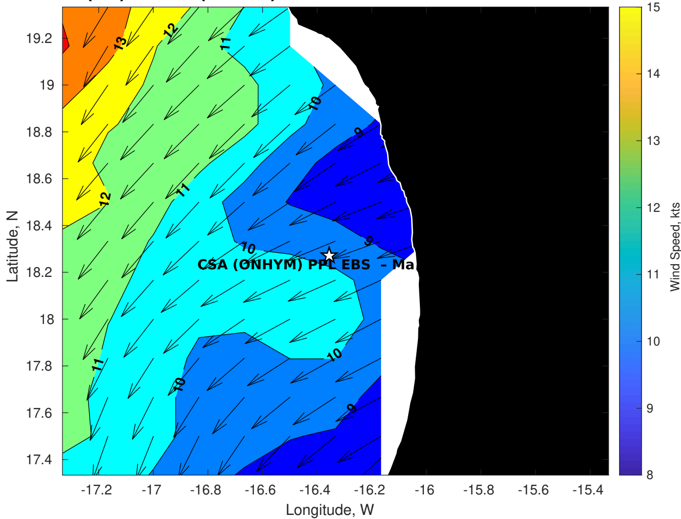
GFS Winds (kts) for CSA (ONHYM) PPL EBS - Mauritania at 01-Feb-2026 09:00:00
