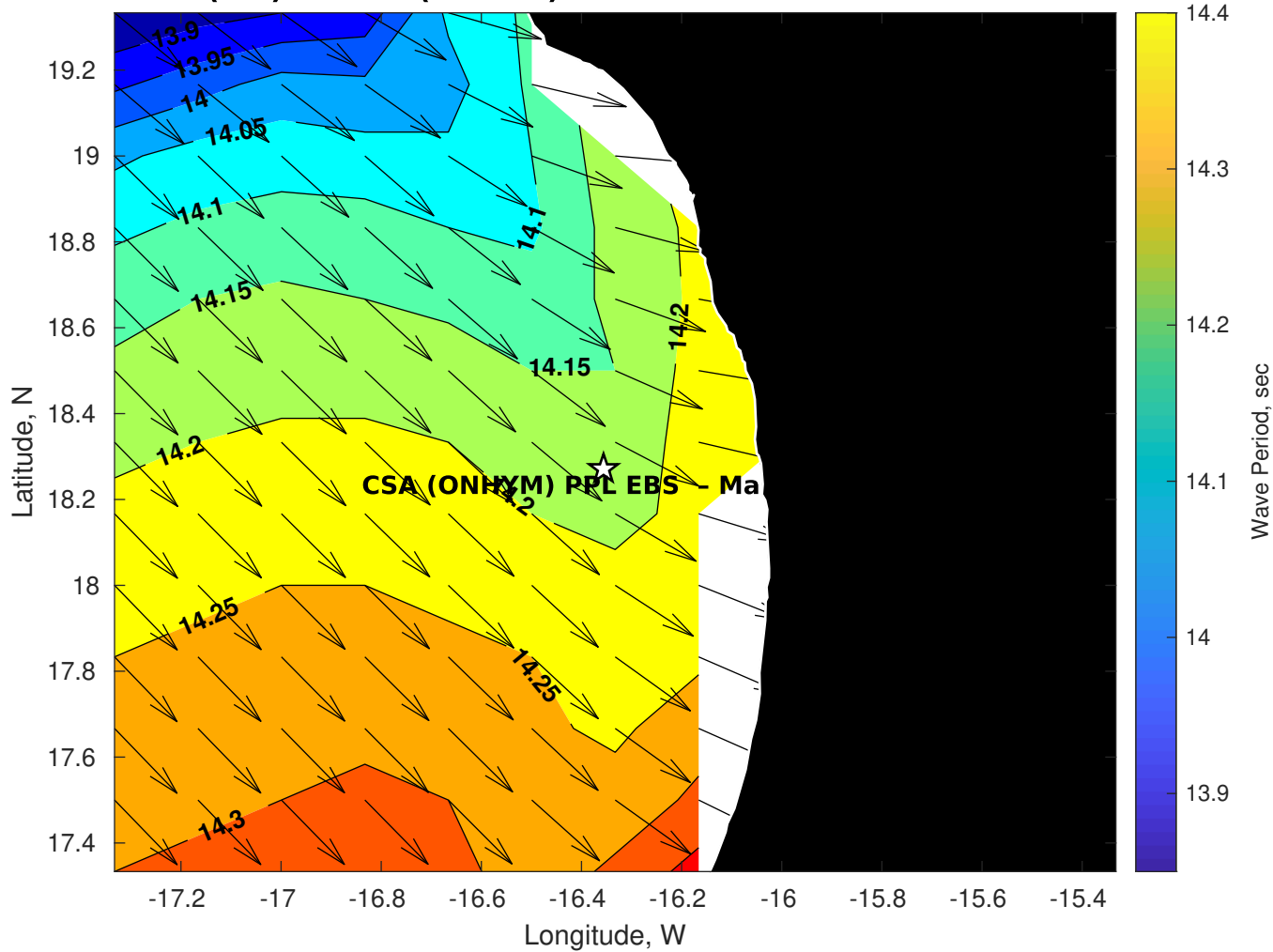
GFS Wave Period (sec) for CSA (ONHYM) PPL EBS - Mauritania at 01-Feb-2026 09:00:00
