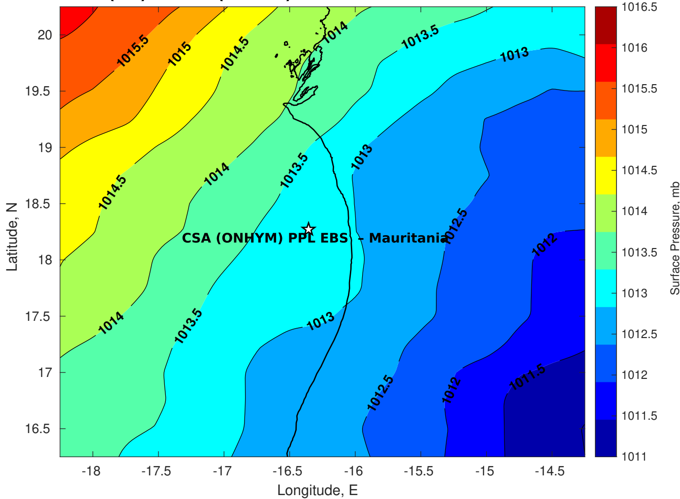
Surface Pressure (mb) for CSA (ONHYM) PPL EBS - Mauritania at 03-Feb-2026 00:00:00
