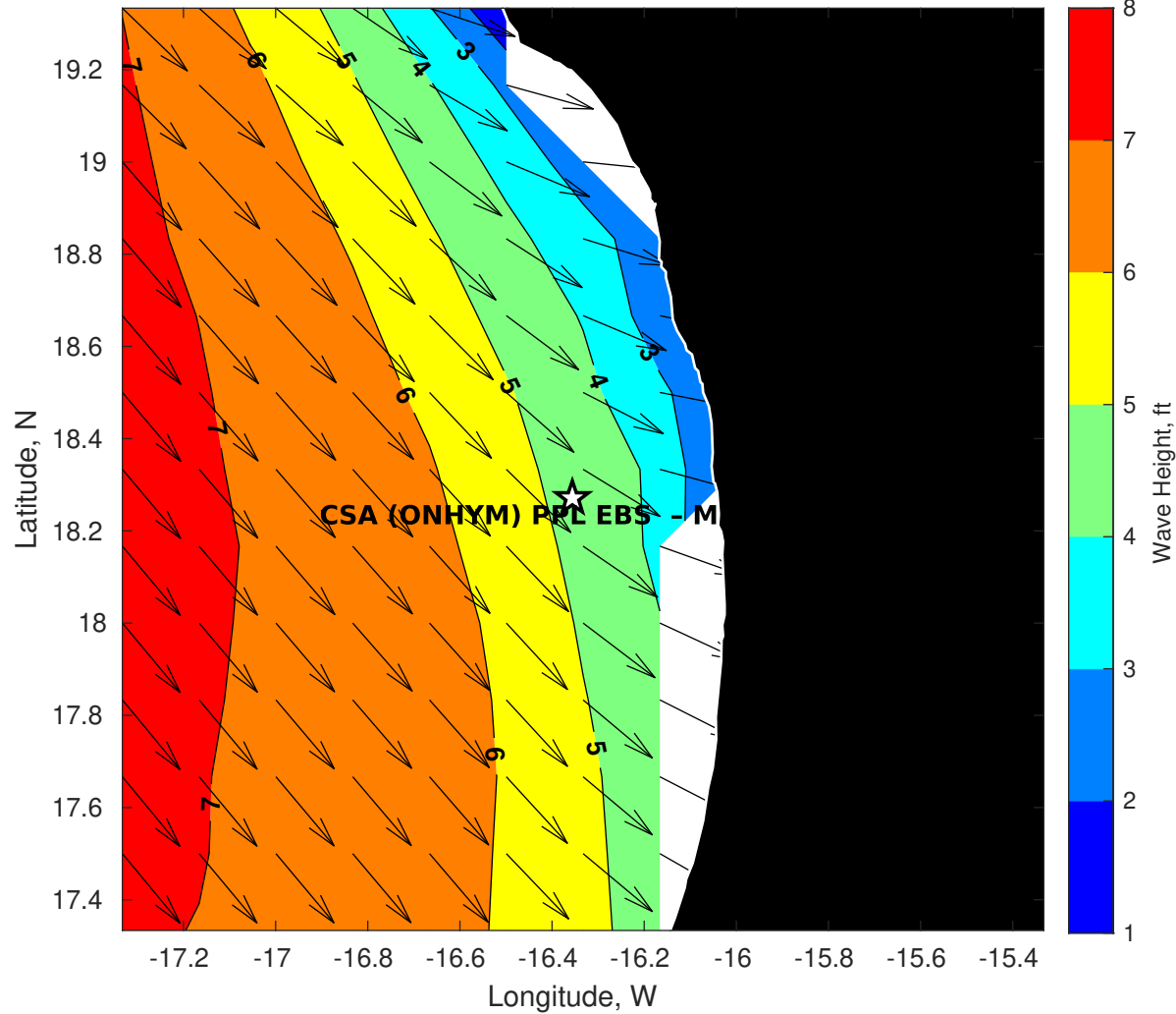
GFS Wave Height (ft) for CSA (ONHYM) PPL EBS - Mauritania at 01-Feb-2026 09:00:00
