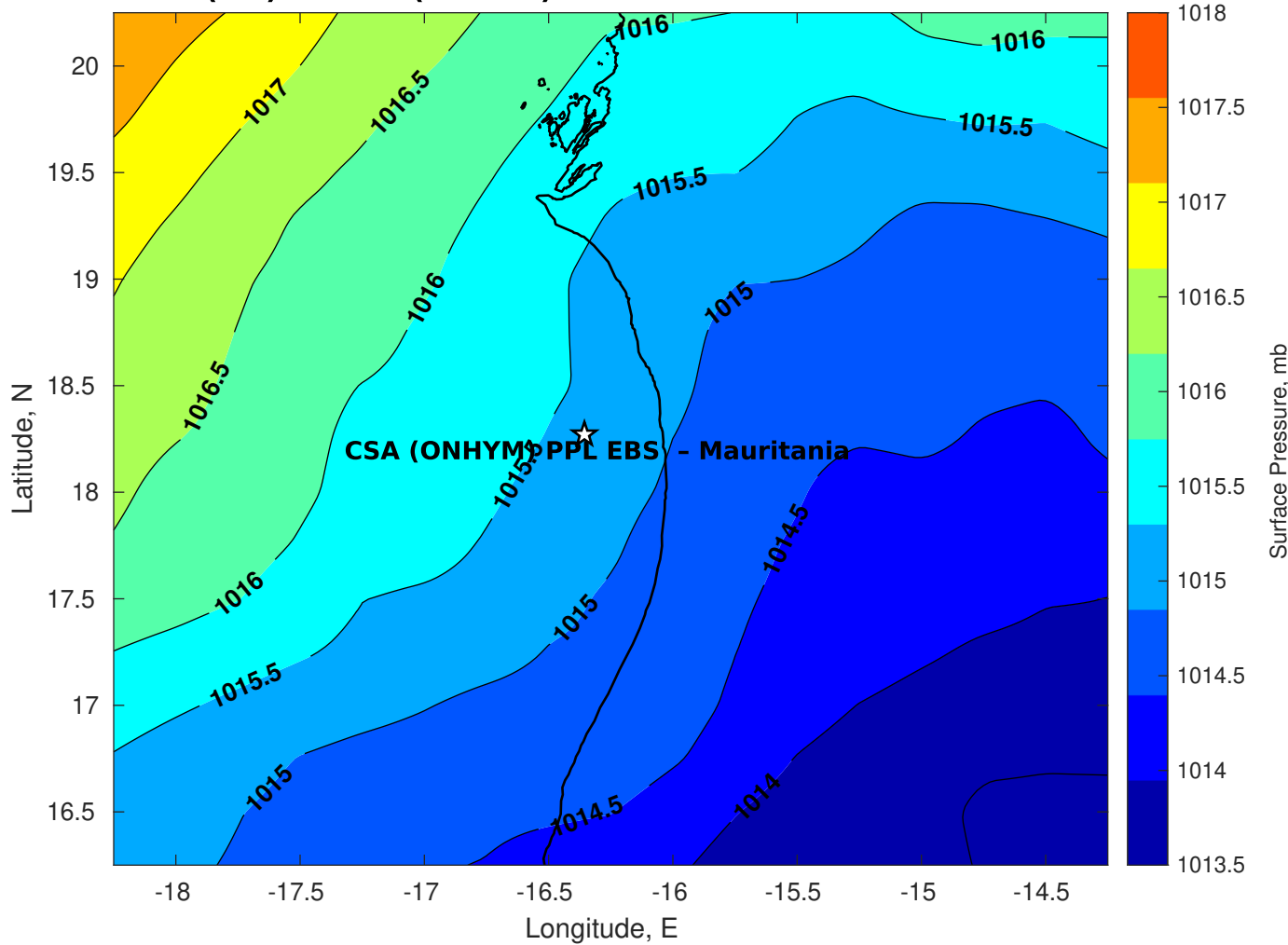
Surface Pressure (mb) for CSA (ONHYM) PPL EBS - Mauritania at 01-Feb-2026 00:00:00
