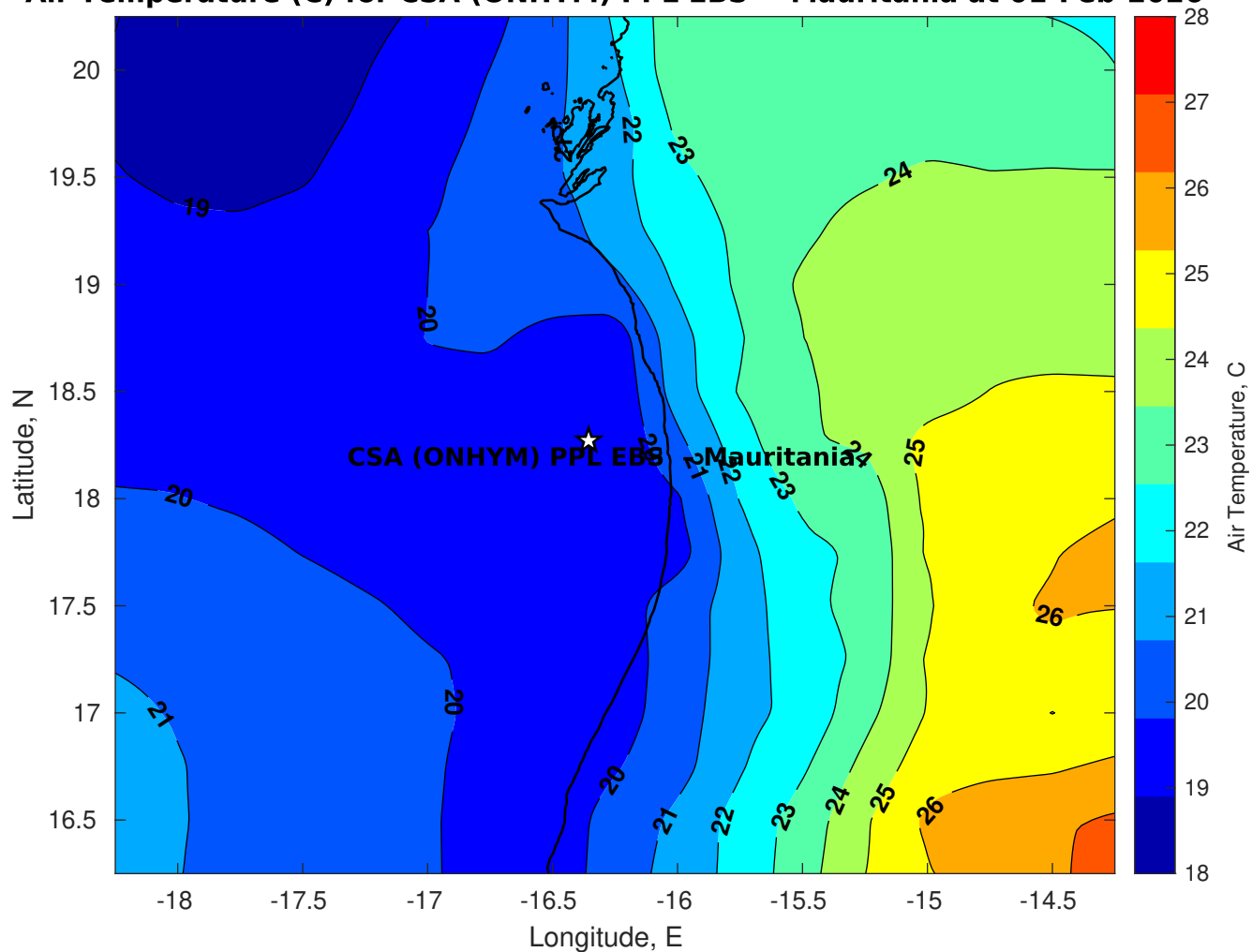
Air Temperature (C) for CSA (ONHYM) PPL EBS - Mauritania at 01-Feb-2026
