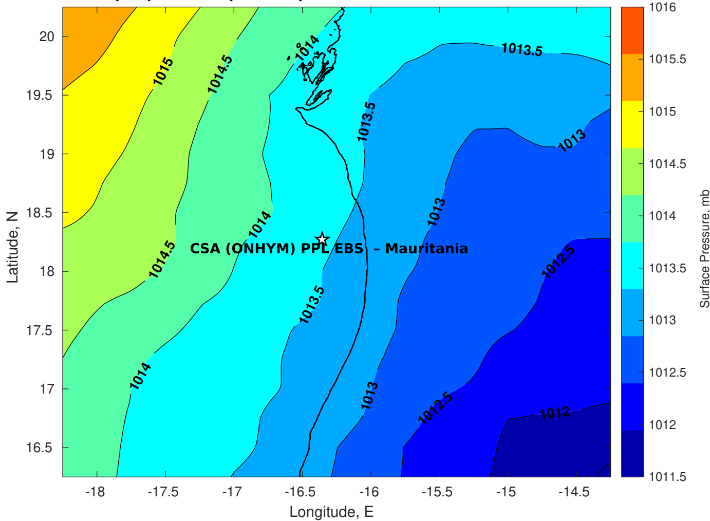
Surface Pressure (mb) for CSA (ONHYM) PPL EBS - Mauritania at 02-Feb-2026 00:00:00
