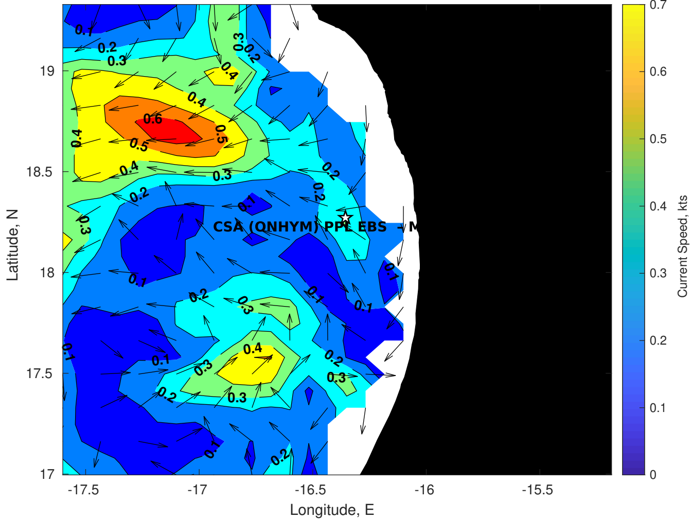
Surface Currents for CSA (ONHYM) PPL EBS - Mauritania at 31-Jan-2026 00:00:00
