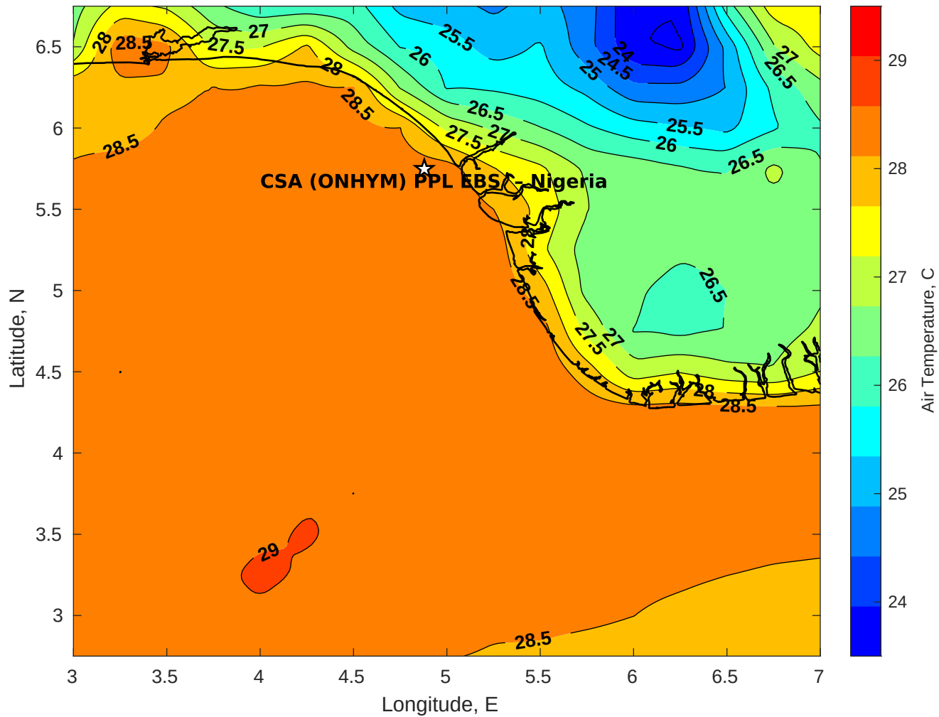
Air Temperature (C) for CSA (ONHYM) PPL EBS - Nigeria at 01-Feb-2026
