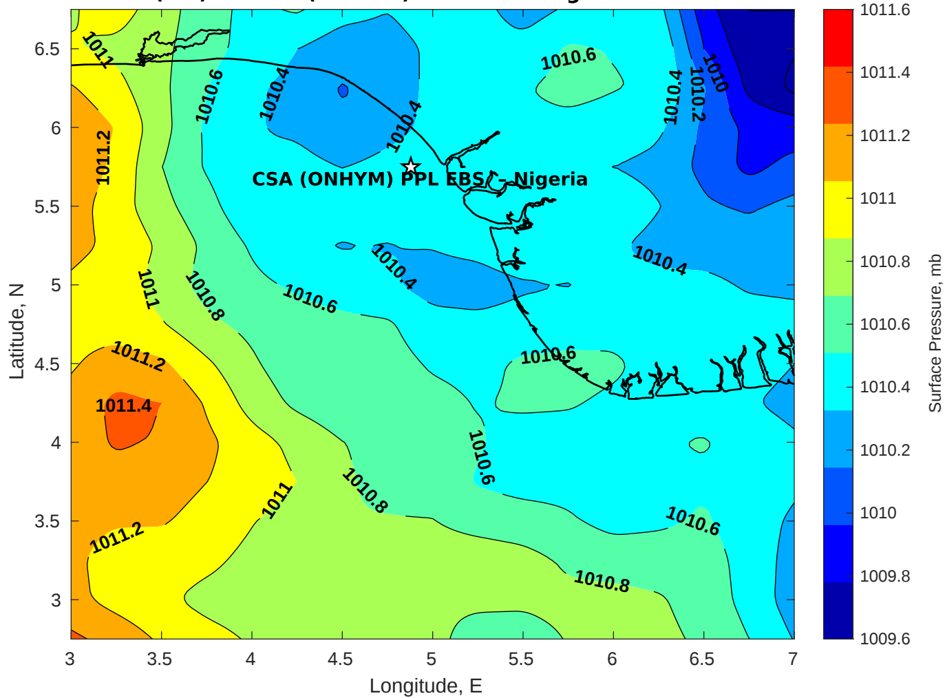
Surface Pressure (mb) for CSA (ONHYM) PPL EBS - Nigeria at 03-Feb-2026 00:00:00
