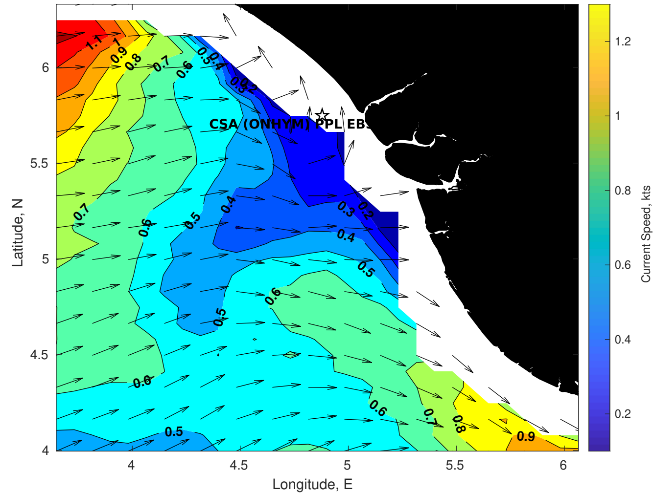
Surface Currents for CSA (ONHYM) PPL EBS - Nigeria at 31-Jan-2026 00:00:00
