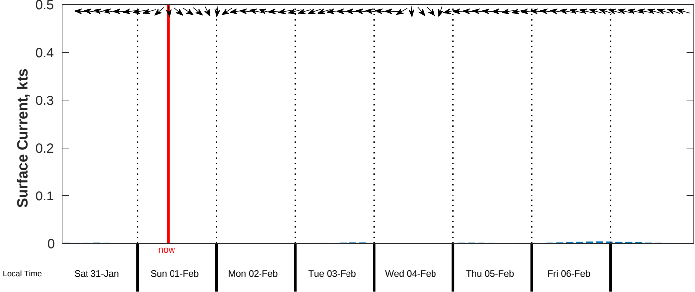
Surface Current Forecast for CSA (ONHYM) PPL EBS - Nigeria from 31-Jan-2026 00:00:00 to 08-Feb-2026 00:00:00
