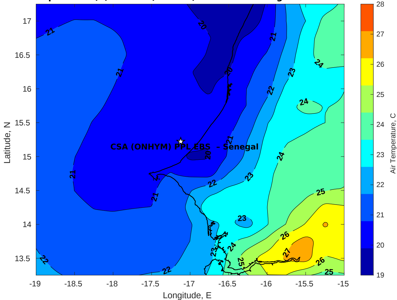
Air Temperature (C) for CSA (ONHYM) PPL EBS - Senegal at 01-Feb-2026
