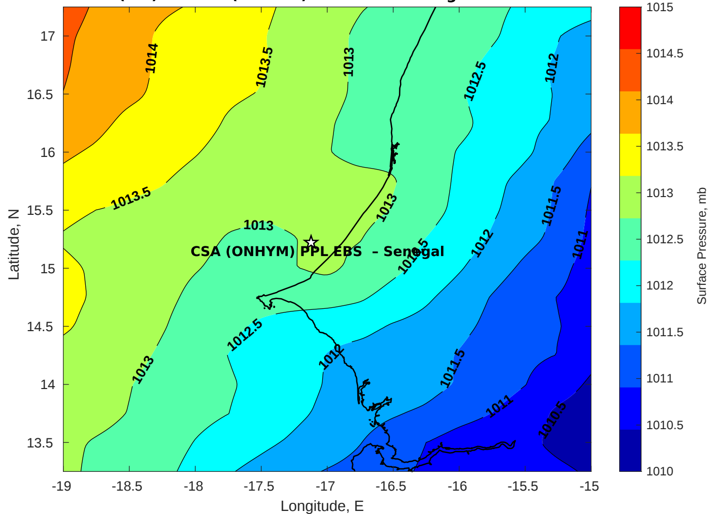
Surface Pressure (mb) for CSA (ONHYM) PPL EBS - Senegal at 03-Feb-2026 00:00:00
