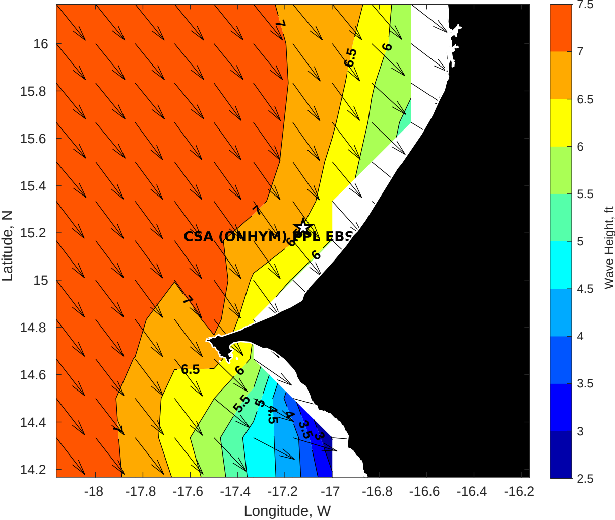
GFS Wave Height (ft) for CSA (ONHYM) PPL EBS - Senegal at 01-Feb-2026 09:00:00
