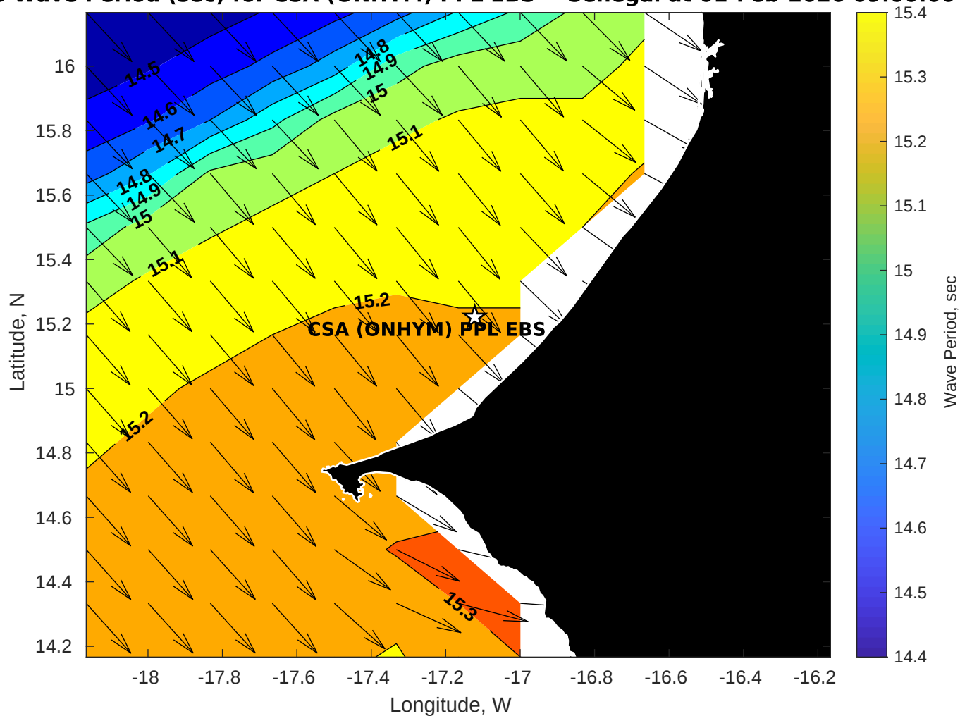
GFS Wave Period (sec) for CSA (ONHYM) PPL EBS - Senegal at 01-Feb-2026 09:00:00
