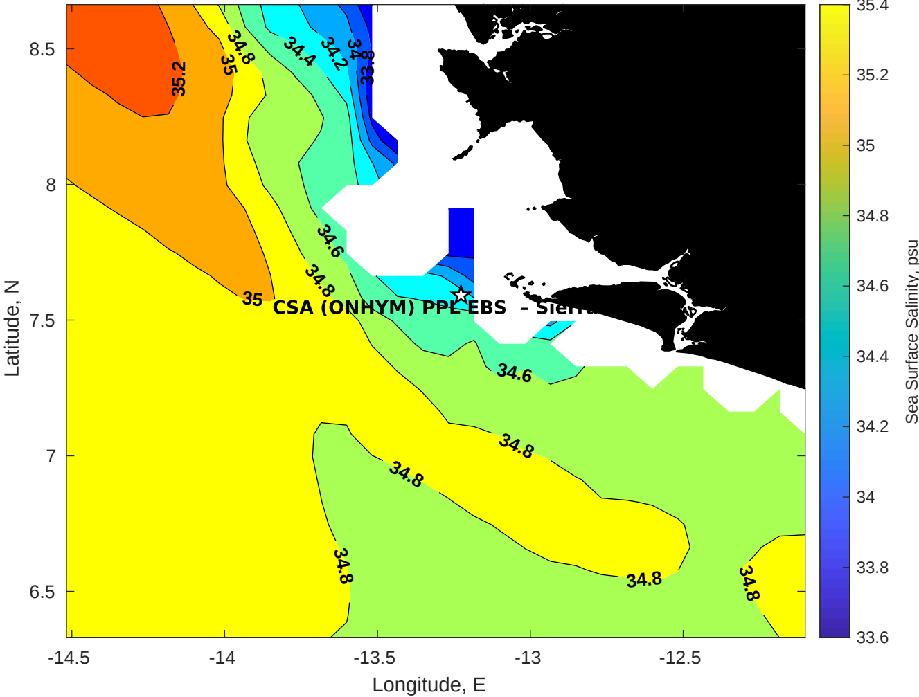
Surface Salinity for CSA (ONHYM) PPL EBS - Sierra Leone at 31-Jan-2026 00:00:00
