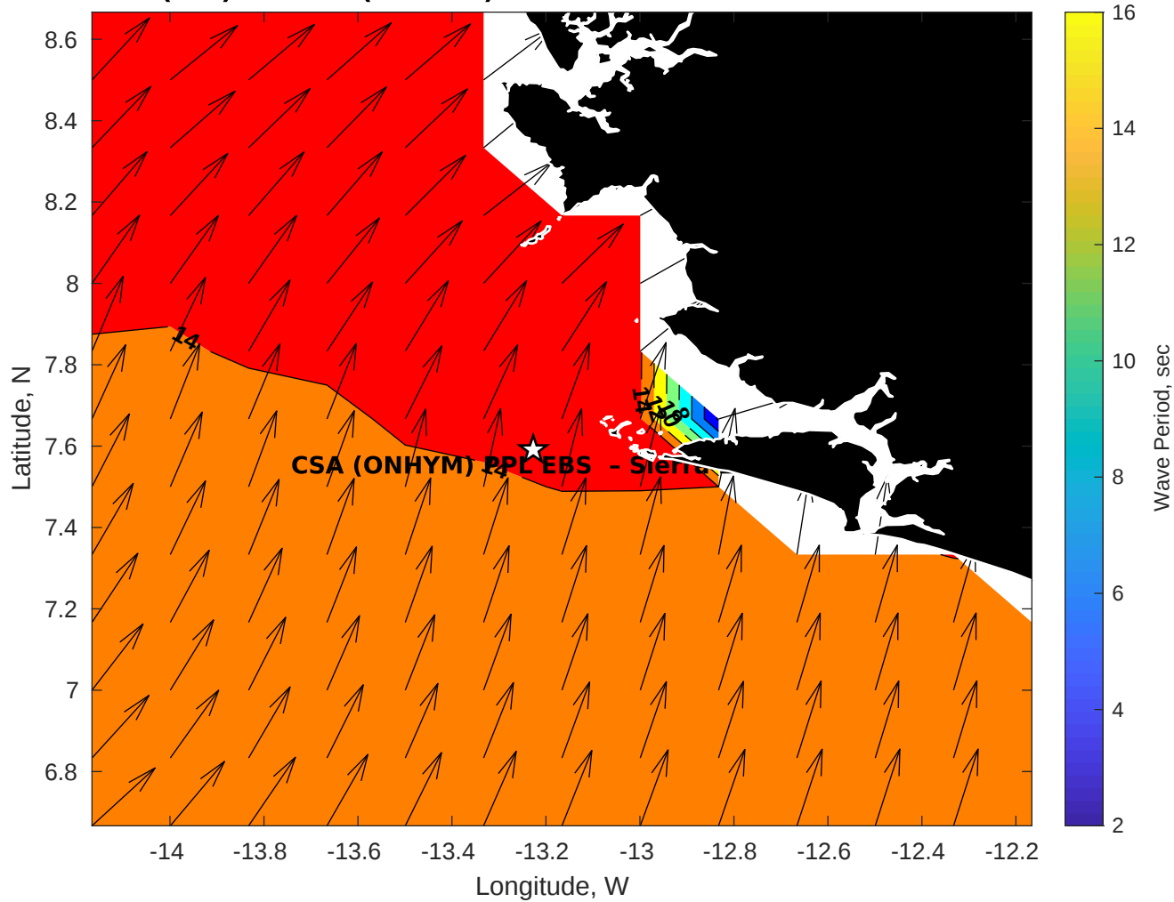
GFS Wave Period (sec) for CSA (ONHYM) PPL EBS - Sierra Leone at 01-Feb-2026 09:00:00
