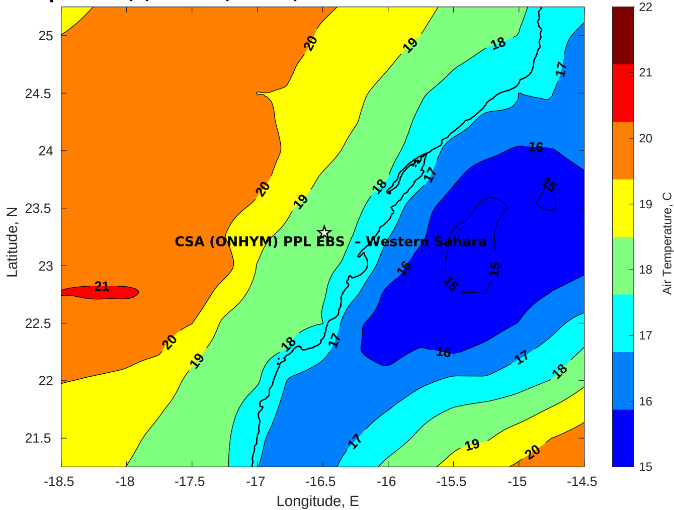
Air Temperature (C) for CSA (ONHYM) PPL EBS - Western Sahara at 01-Feb-2026
