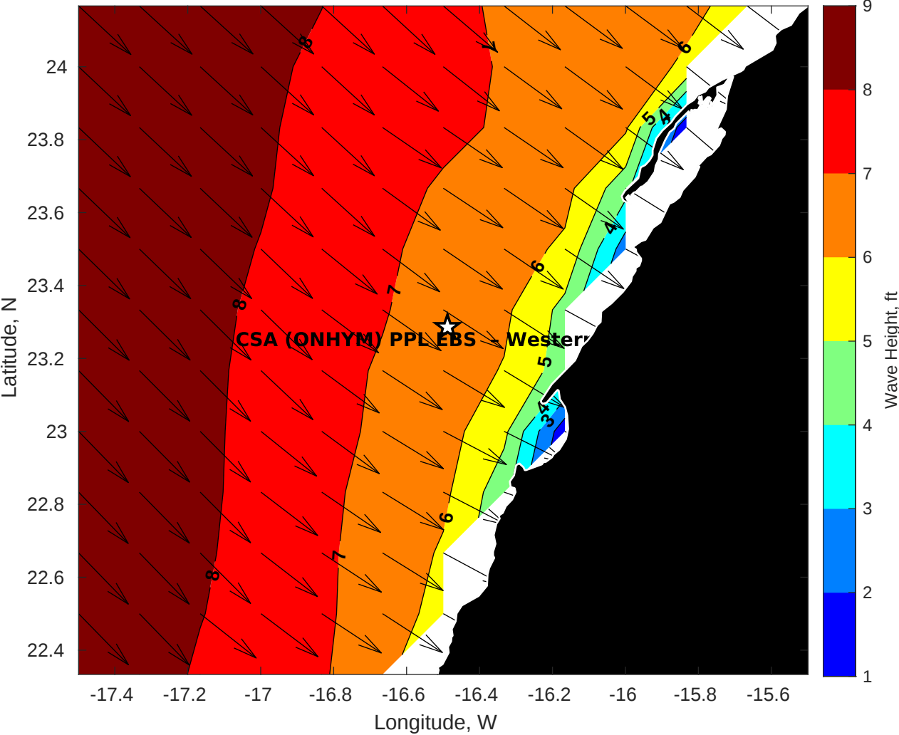
GFS Wave Height (ft) for CSA (ONHYM) PPL EBS - Western Sahara at 01-Feb-2026 09:00:00
