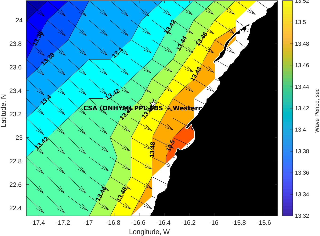
GFS Wave Period (sec) for CSA (ONHYM) PPL EBS - Western Sahara at 01-Feb-2026 09:00:00
