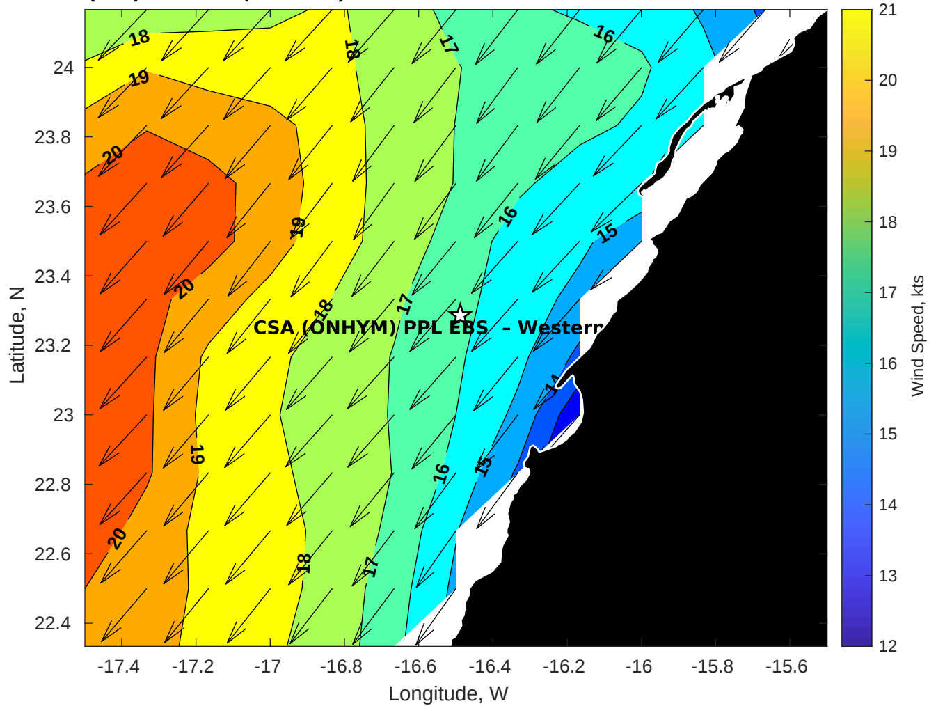
GFS Winds (kts) for CSA (ONHYM) PPL EBS - Western Sahara at 01-Feb-2026 09:00:00
