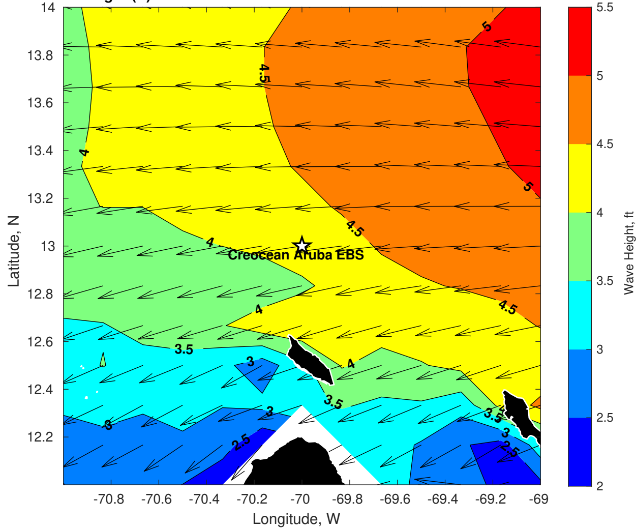
GFS Wave Height (ft) for Creoccean Aruba EBS at 01-Feb-2026 09:00:00
