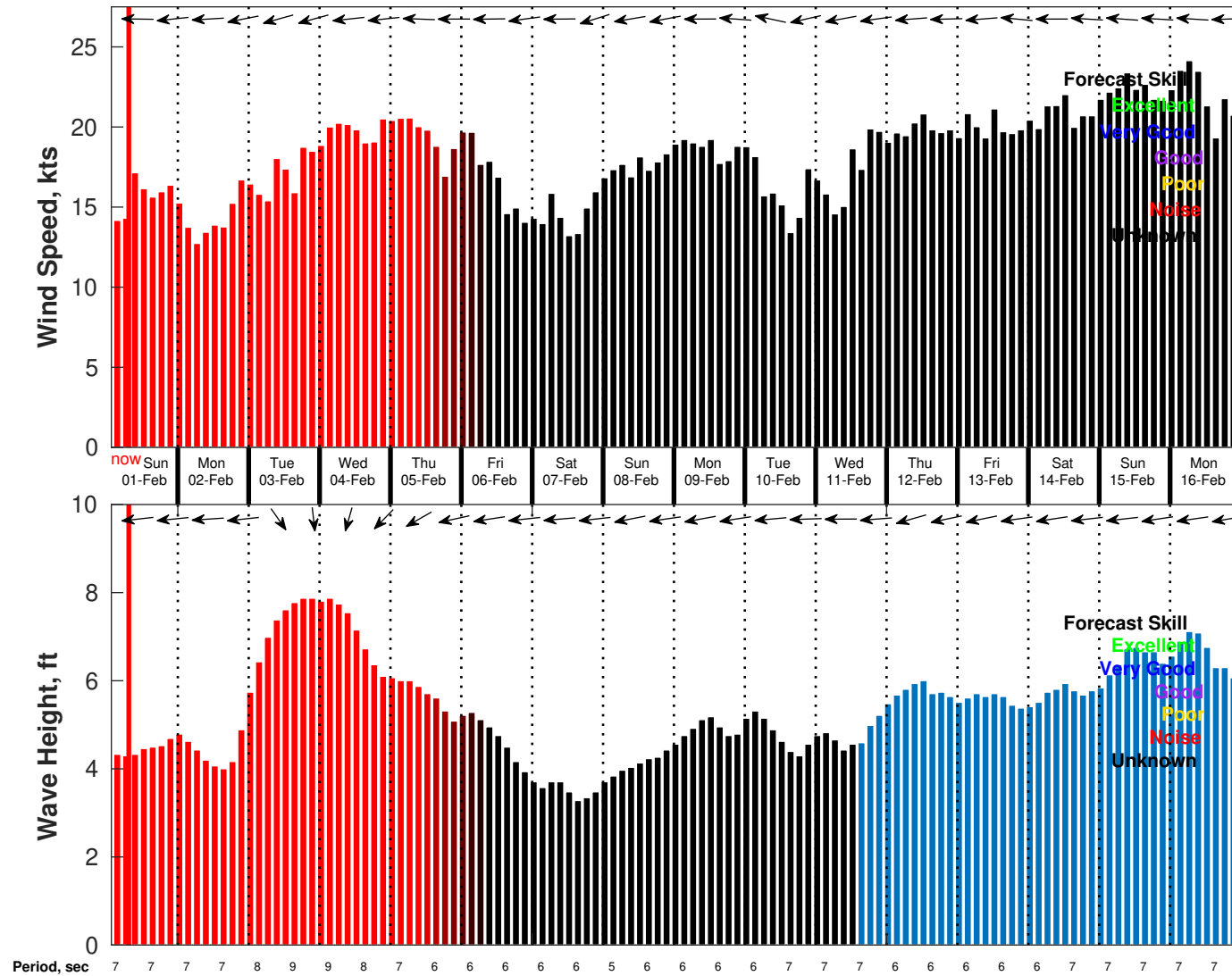
Wind & Wave Forecast for Creocan Aruba EBS from 01-Feb-2026 02:00:00 to 17-Feb-2026 02:00:00
