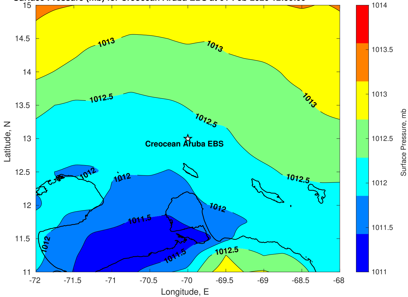
Surface Pressure (mb) for Creoccean Aruba EBS at 01-Feb-2026 12:00:00
