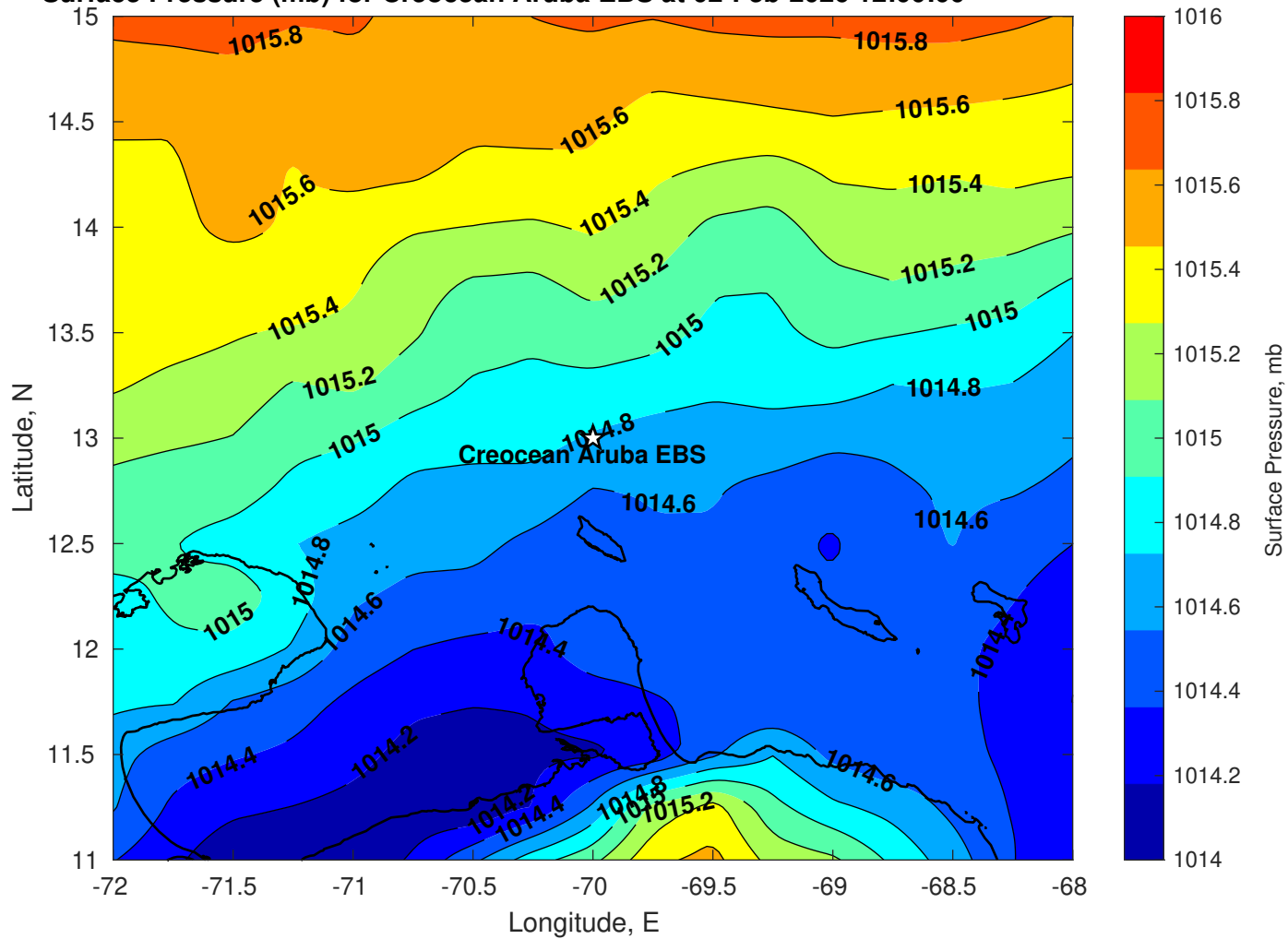
Surface Pressure (mb) for Creoccean Aruba EBS at 02-Feb-2026 12:00:00
