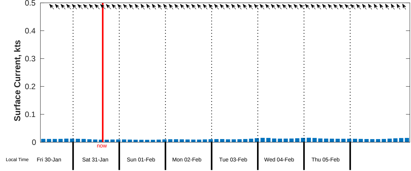
Surface Current Forecast for Creocean Aruba EBS from 31-Jan-2026 00:00:00 to 08-Feb-2026 00:00:00
