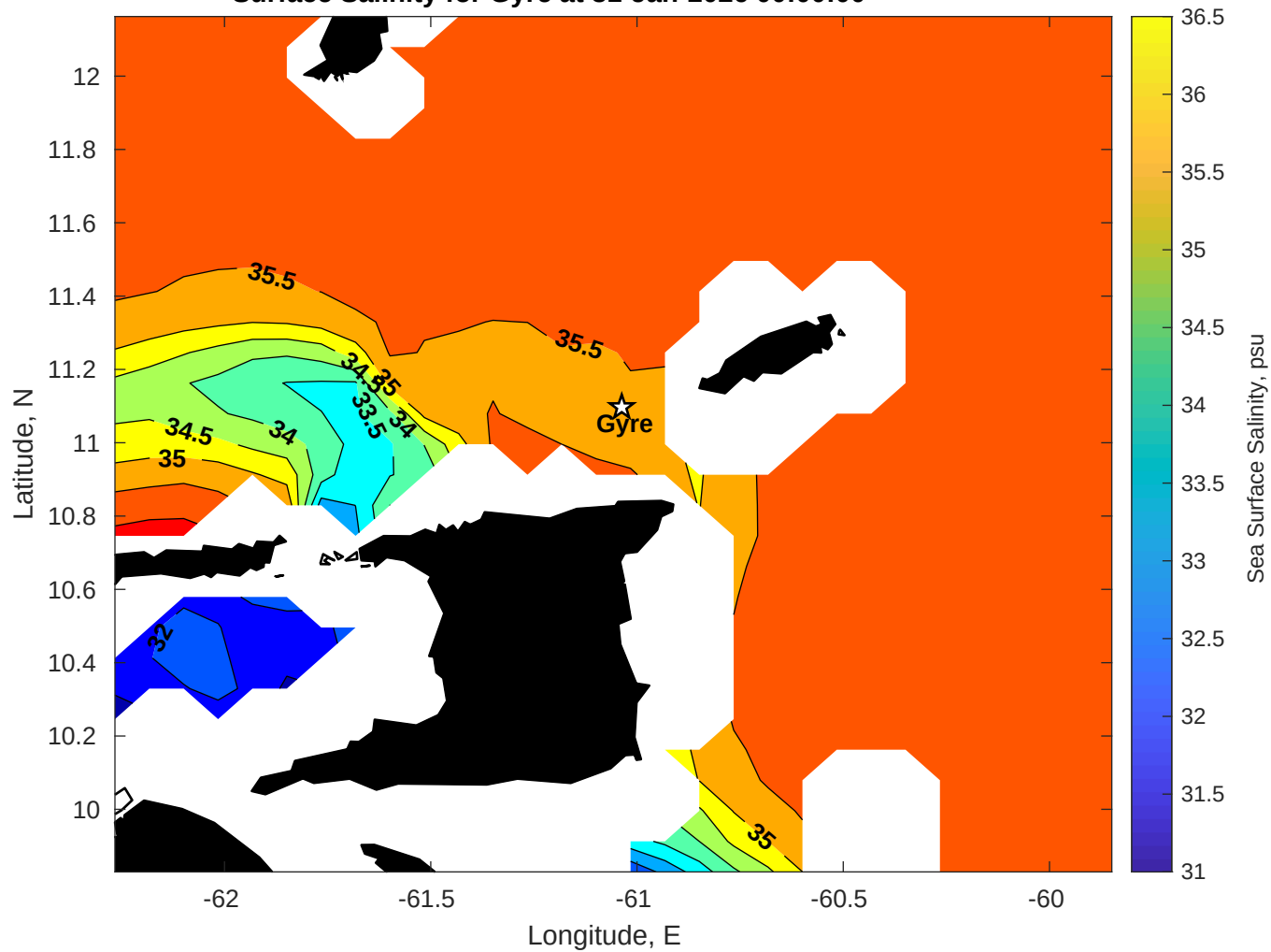
Surface Salinity for Gyre at 31-Jan-2026 00:00:00
