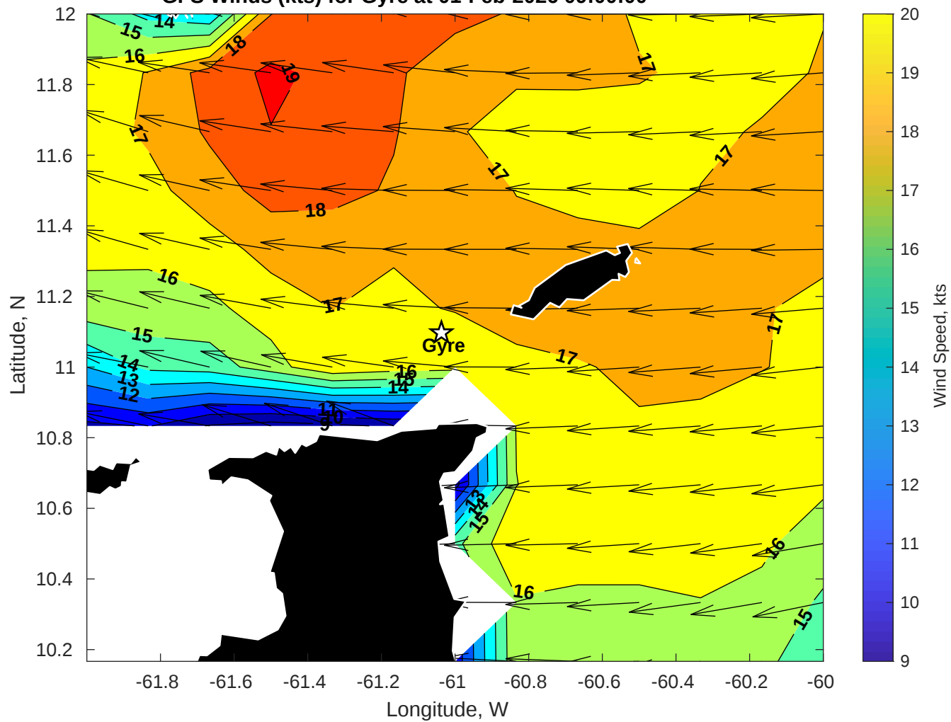
GFS Winds (kts) for Gyre at 01-Feb-2026 09:00:00
