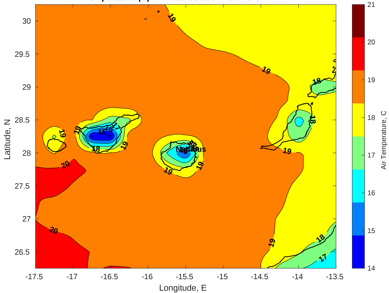
Air Temperature (C) for Nautilus at 01-Feb-2026
