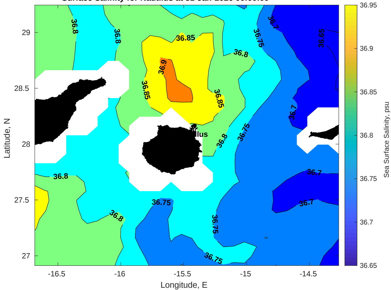
Surface Salinity for Nautilus at 31-Jan-2026 00:00:00
