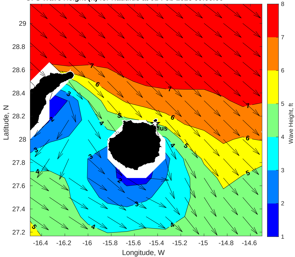
GFS Wave Height (ft) for Nautilus at 01-Feb-2026 09:00:00
