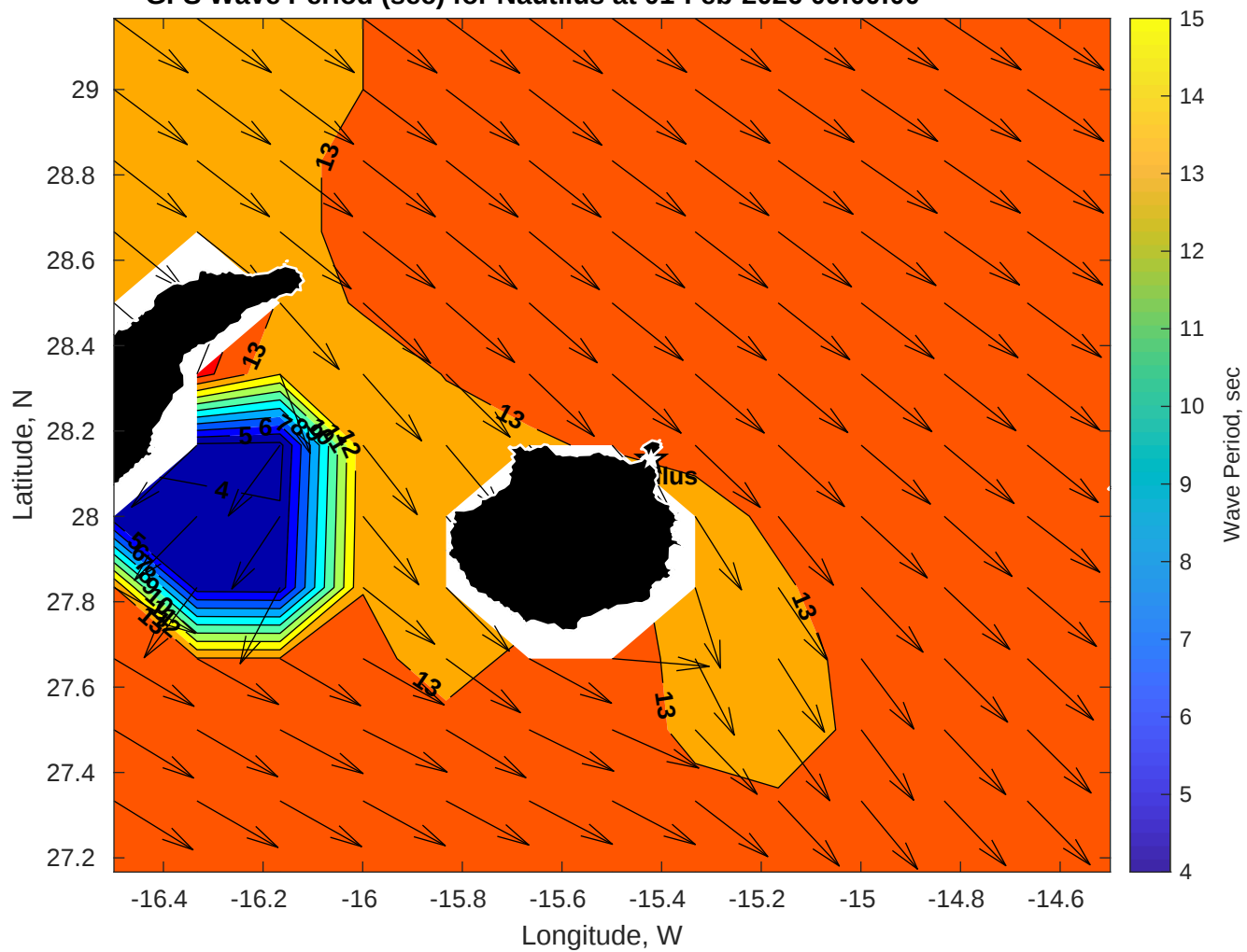
GFS Wave Period (sec) for Nautilus at 01-Feb-2026 09:00:00
