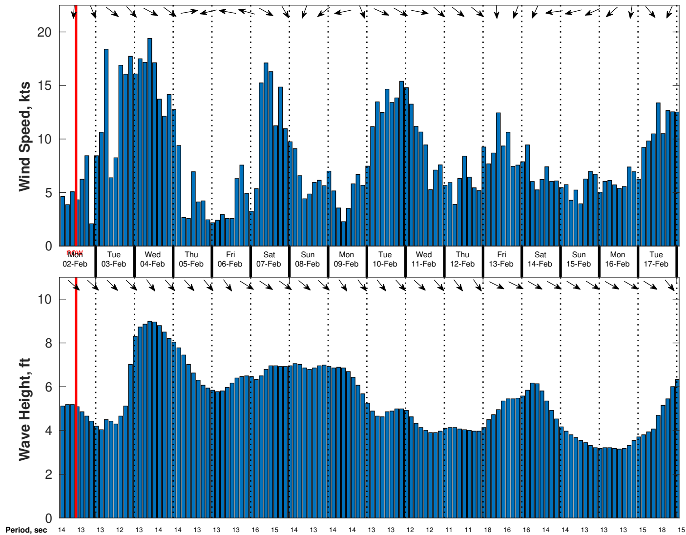
Wind & Wave Forecast for Nautilus from 01-Feb-2026 02:00:00 to 17-Feb-2026 02:00:00
