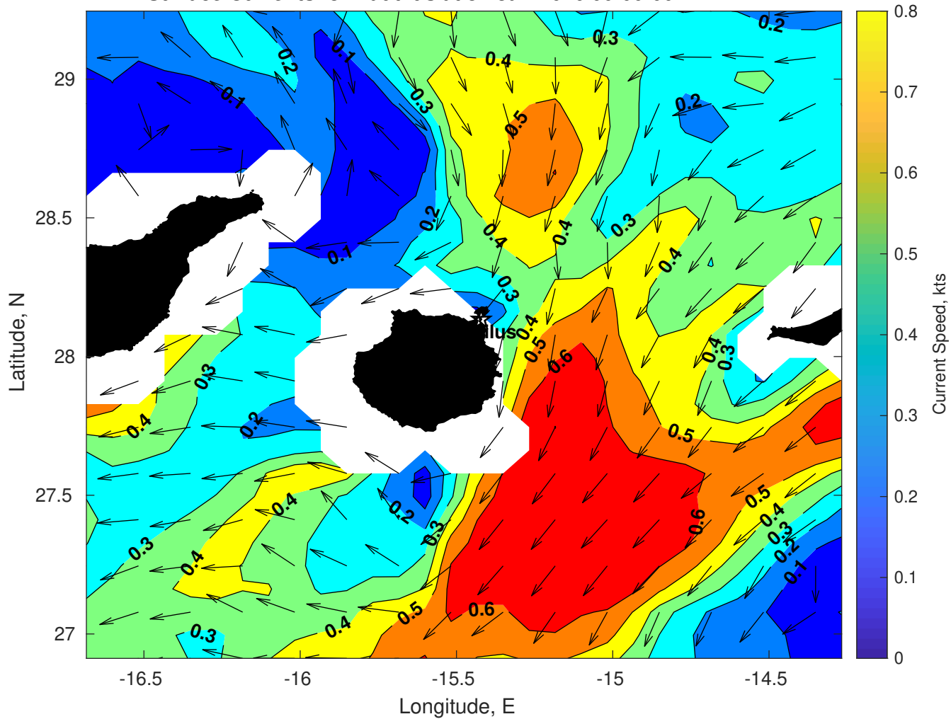
Surface Currents for Nautilus at 31-Jan-2026 00:00:00
