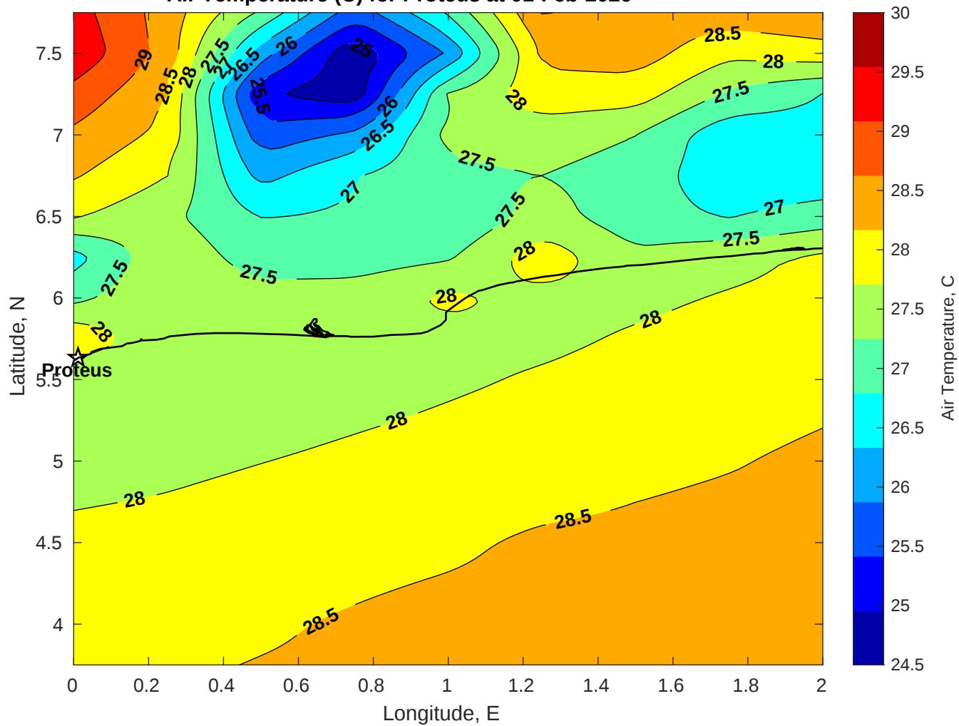
Air Temperature (C) for Proteus at 01-Feb-2026
