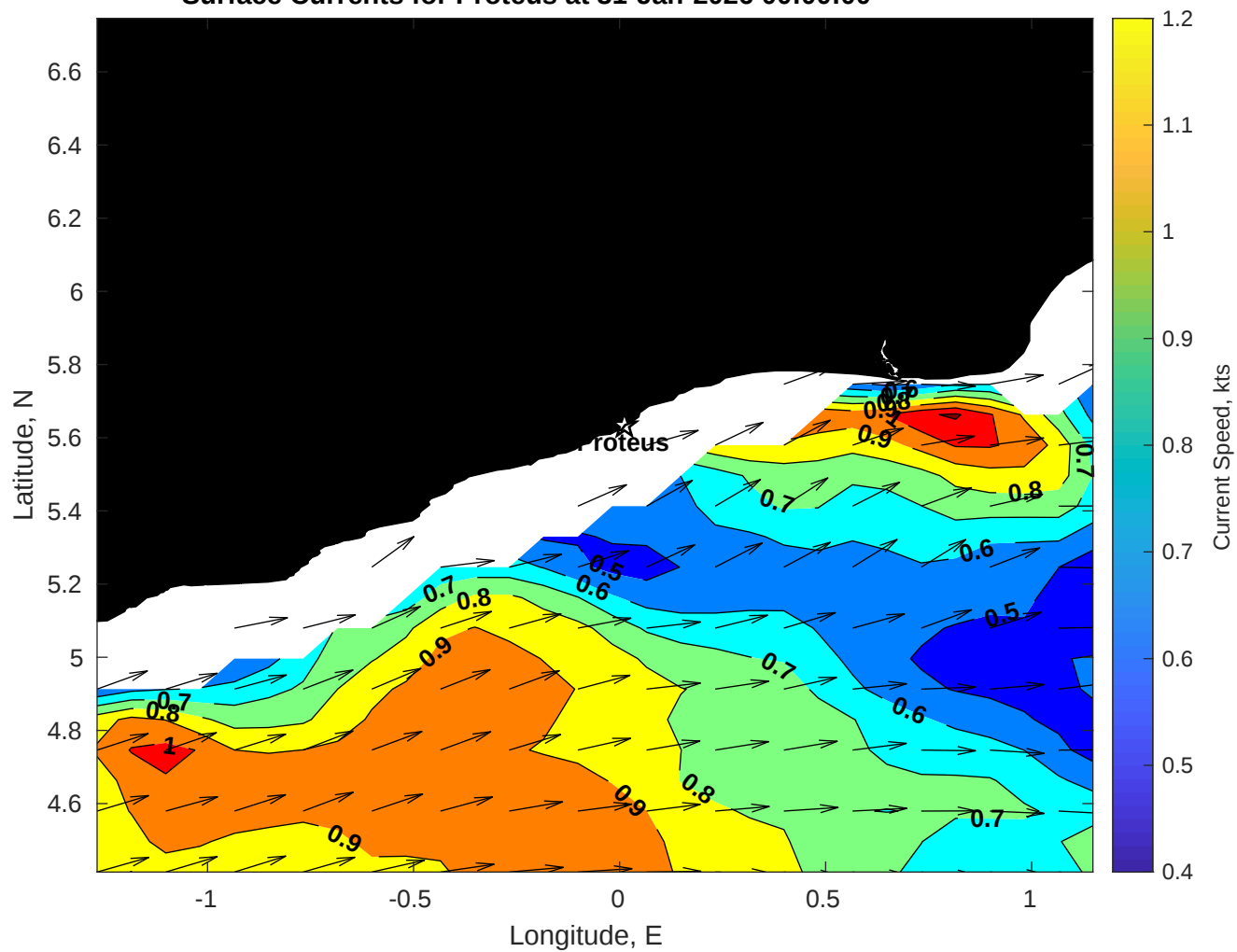
Surface Currents for Proteus at 31-Jan-2026 00:00:00
