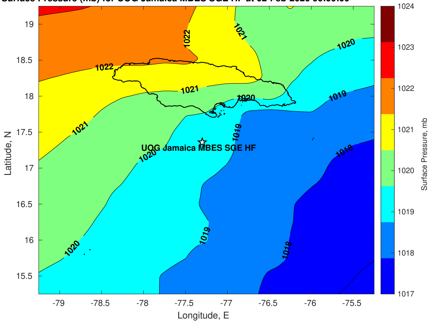
Surface Pressure (mb) for UOG Jamaica MBES SGE HF at 02-Feb-2026 06:00:00
