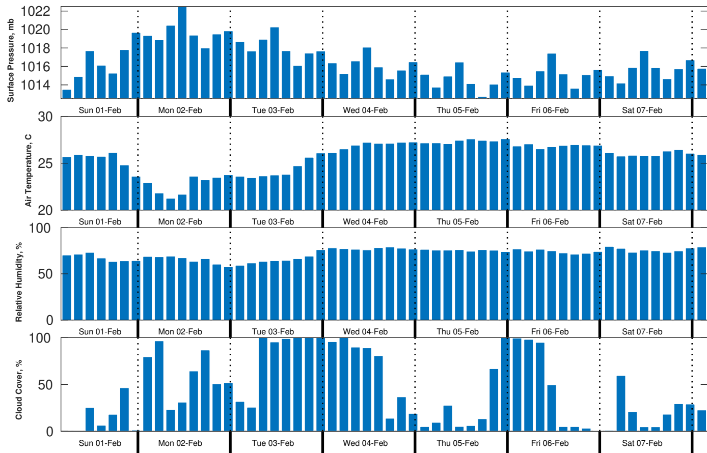
Met Forecast for UOG Jamaica MBES SGE HF from 01-Feb-2026 06:00:00 to 08-Feb-2026 06:00:00
