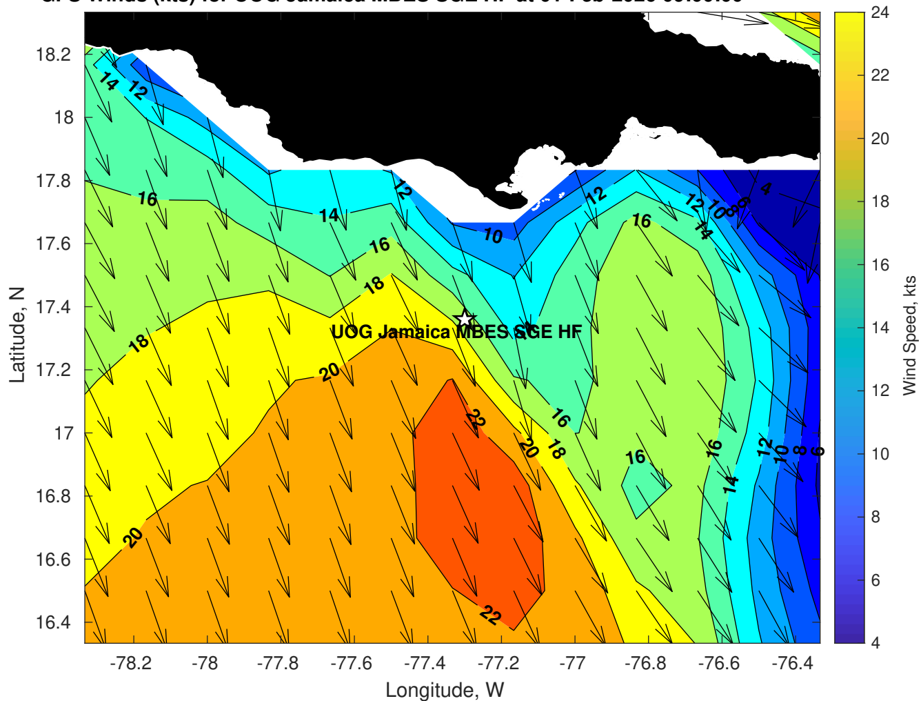
GFS Winds (kts) for UOG Jamaica MBES SGE HF at 01-Feb-2026 09:00:00
