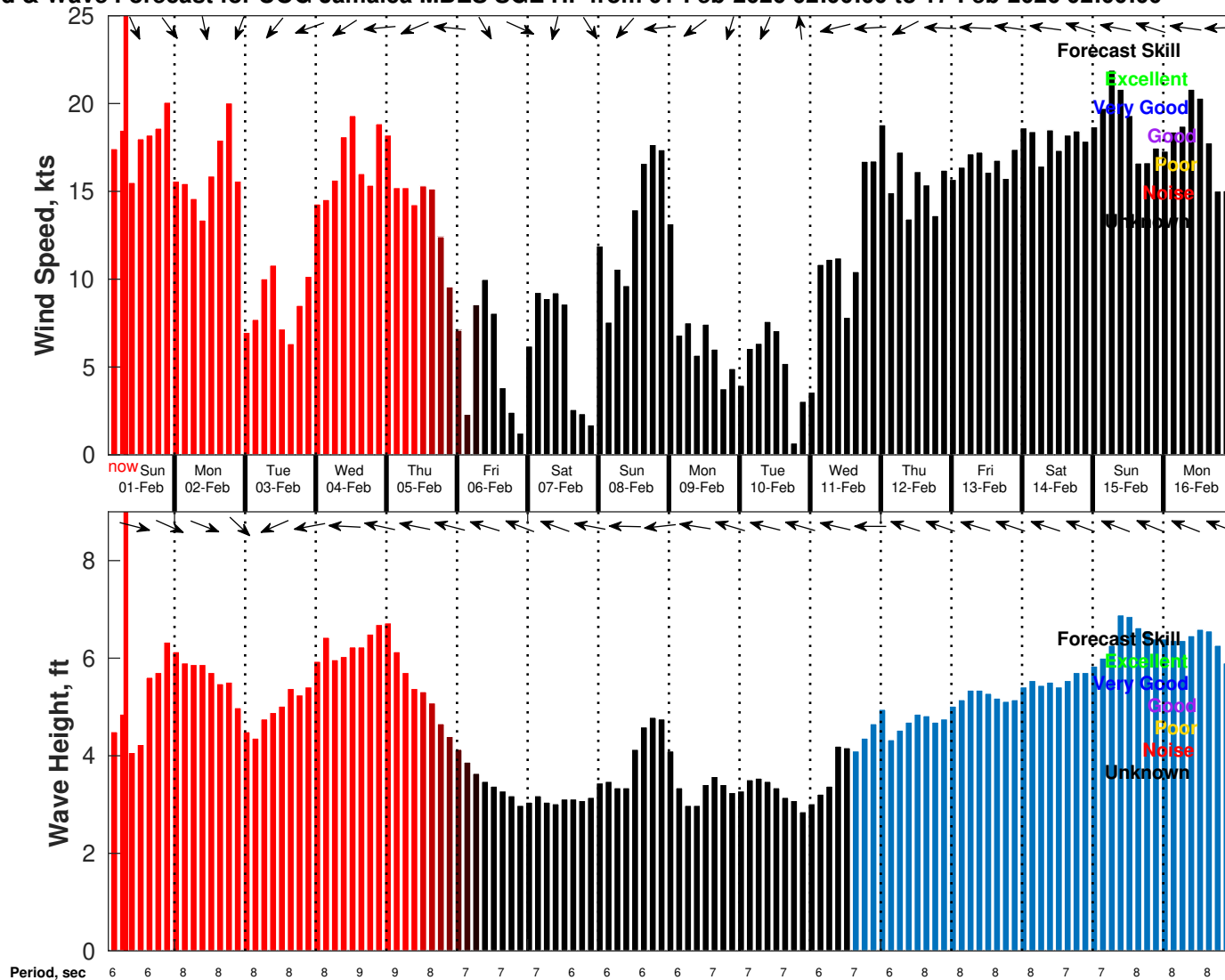
Wind & Wave Forecast for UOG Jamaica MBES SGE HF from 01-Feb-2026 02:00:00 to 17-Feb-2026 02:00:00
