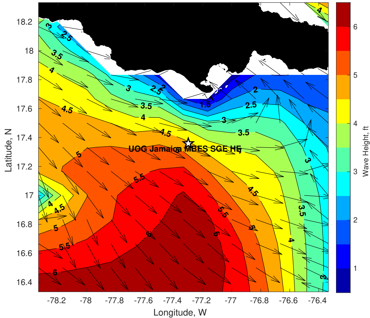
GFS Wave Height (ft) for UOG Jamaica MBES SGE HF at 01-Feb-2026 09:00:00
