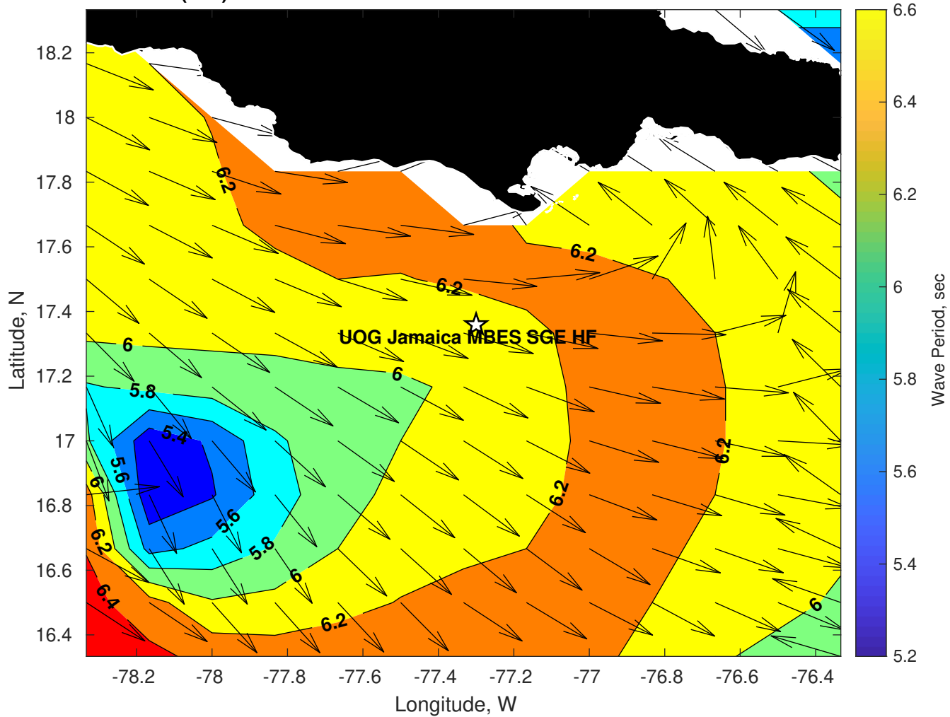
GFS Wave Period (sec) for UOG Jamaica MBES SGE HF at 01-Feb-2026 09:00:00
