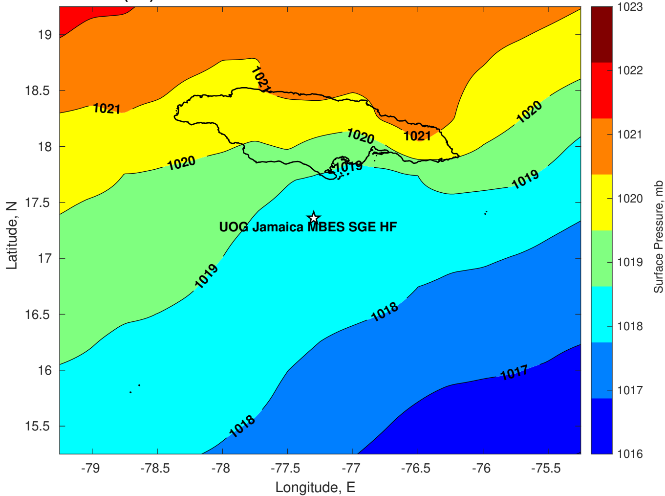
Surface Pressure (mb) for UOG Jamaica MBES SGE HF at 03-Feb-2026 06:00:00
