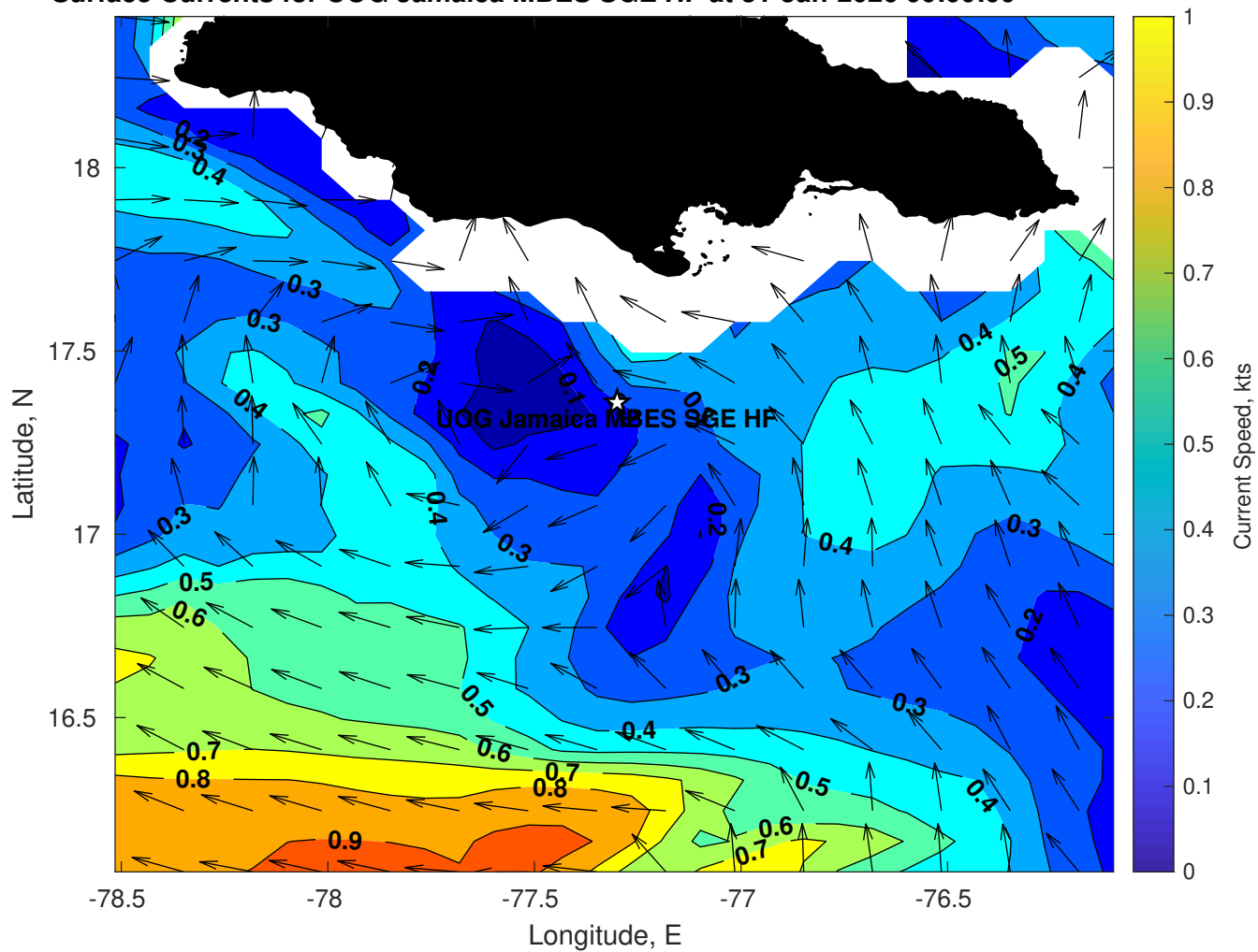
Surface Currents for UOG Jamaica MBES SGE HF at 31-Jan-2026 00:00:00
