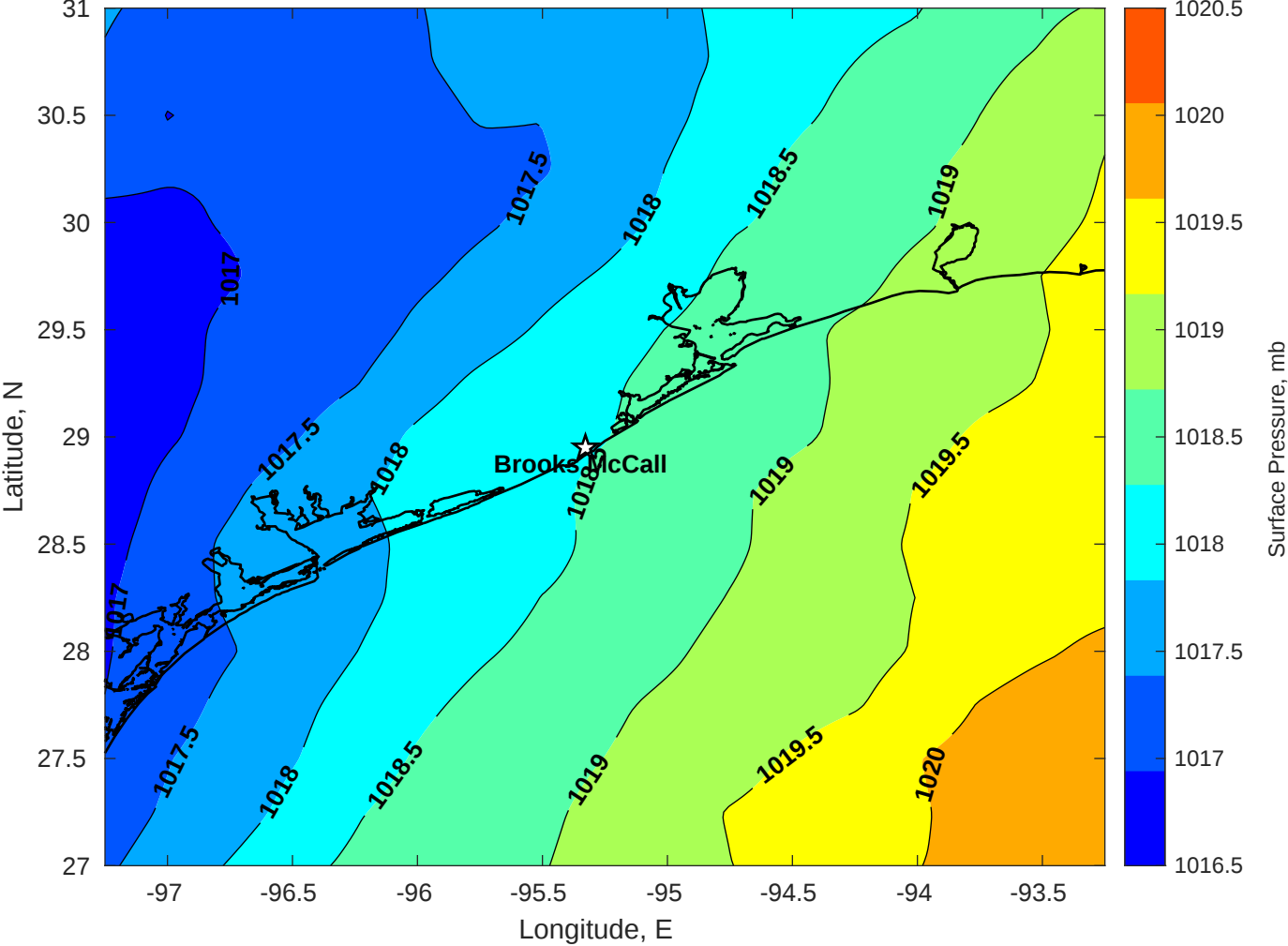
Surface Pressure (mb) for Brooks McCall at 04-Feb-2026 00:00:00
