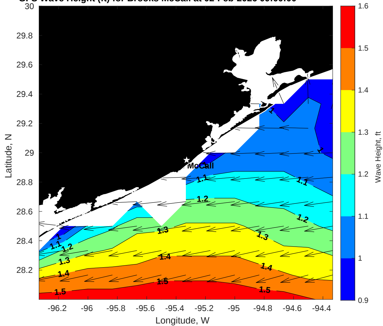
GFS Wave Height (ft) for Brooks McCall at 02-Feb-2026 09:00:00
