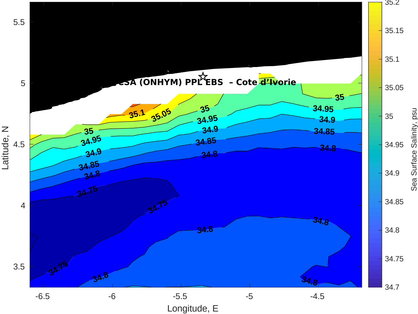
Surface Salinity for CSA (ONHYM) PPL EBS - Cote d'Ivoire at 01-Feb-2026 00:00:00
