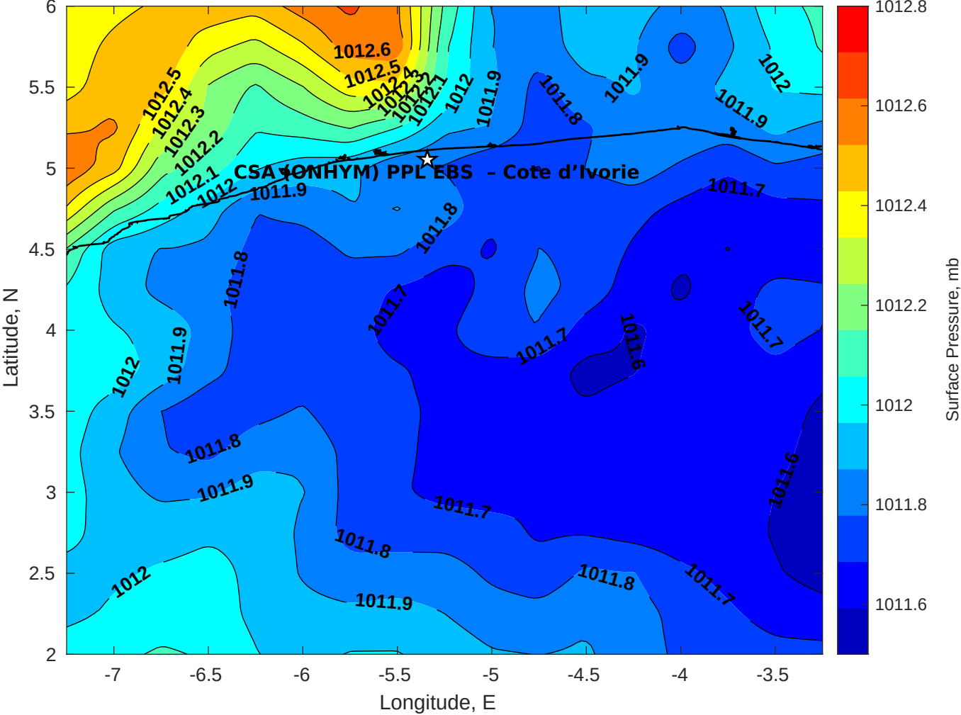
Surface Pressure (mb) for CSA (ONHYM) PPL EBS - Cote d'Ivoire at 03-Feb-2026 00:00:00
