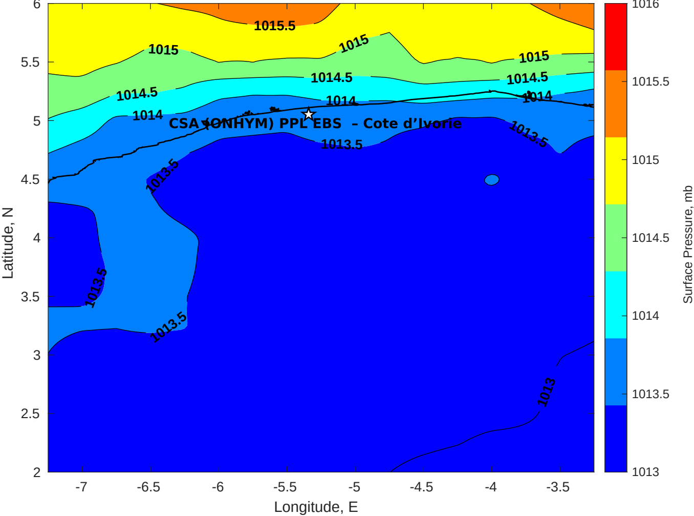
Surface Pressure (mb) for CSA (ONHYM) PPL EBS - Cote d'Ivoire at 04-Feb-2026 00:00:00
