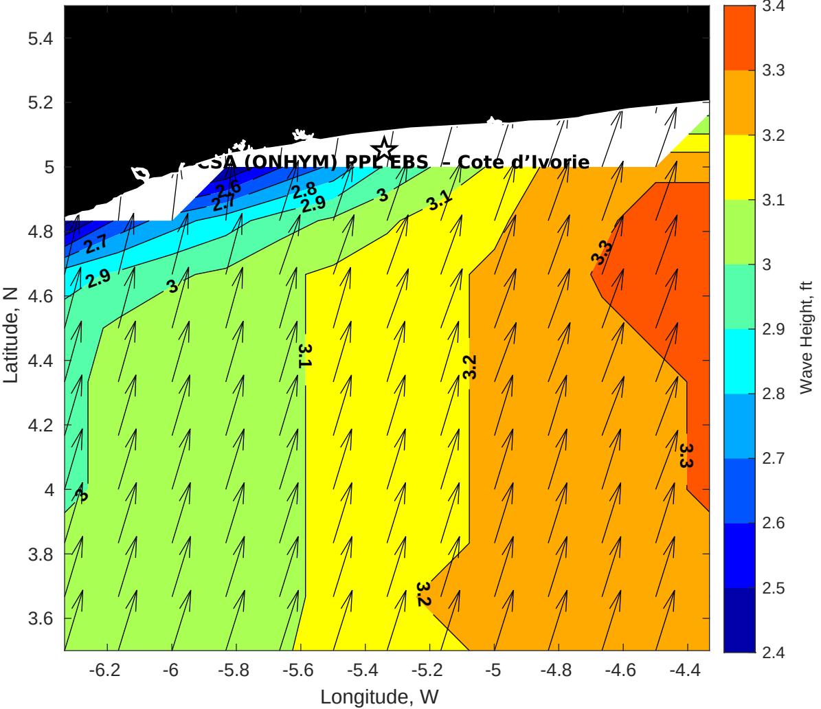
GFS Wave Height (ft) for CSA (ONHYM) PPL EBS - Cote d'Ivoire at 02-Feb-2026 09:00:00
